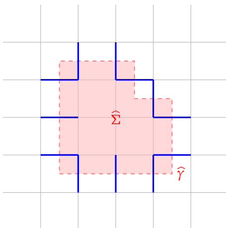
Figure 4: Configuration of the membrane operator U(\widehat{\Sigma}) . Here \widehat{\Sigma} is the red region, and its boundary (represented by the red dashed line) is the curve \widehat{\gamma} on the dual lattice. Those links \langle v, v' \rangle having a non-trivial intersection with \widehat{\gamma} , i.e., (\langle v, v' \rangle, \widehat{\gamma}) = 1 , are shown in blue.
