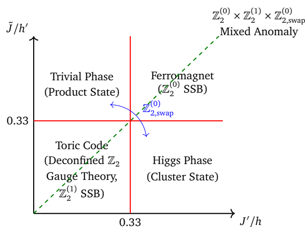
Figure 5: Phase diagram of (50). The Hamiltonian on the green dashed line has an anomaly, separating the trivial and Higgs phases.
