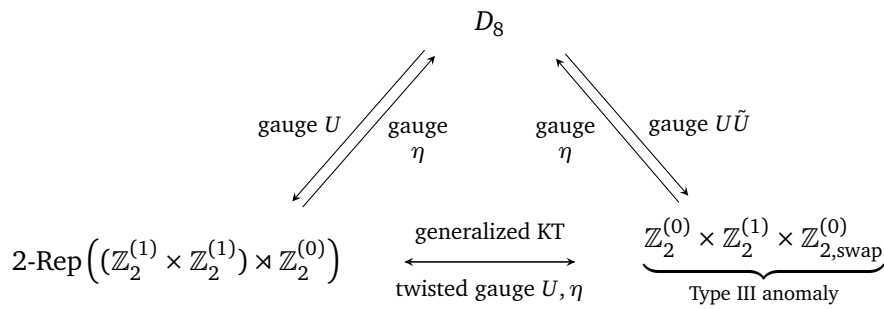
Figure 6: The generalized symmetries in the three models are related by (twisted) gauging.
