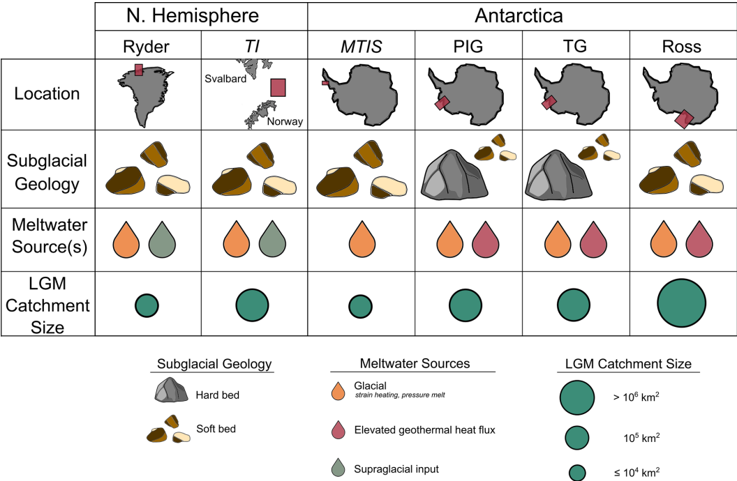
Figure 1. Graphical map illustrating components within a glacial catchment that may influence grain shape alteration and meltwater production compared between study sites. Subglacial geology is binarized into either hard (i.e., crystalline bedrock) or soft (clastic or sedimentary) beds. Relict glacial catchments and deglaciatiated setting names are italicized. TI is for Thor Iversenbanken, MTIS is for Marguerite Trough Ice Stream, PIG is for Pine Island Glacier, TG is for Thwaites Glacier, Ross is for the western Ross Sea, and LGM is for the Last Glacial Maximum.
