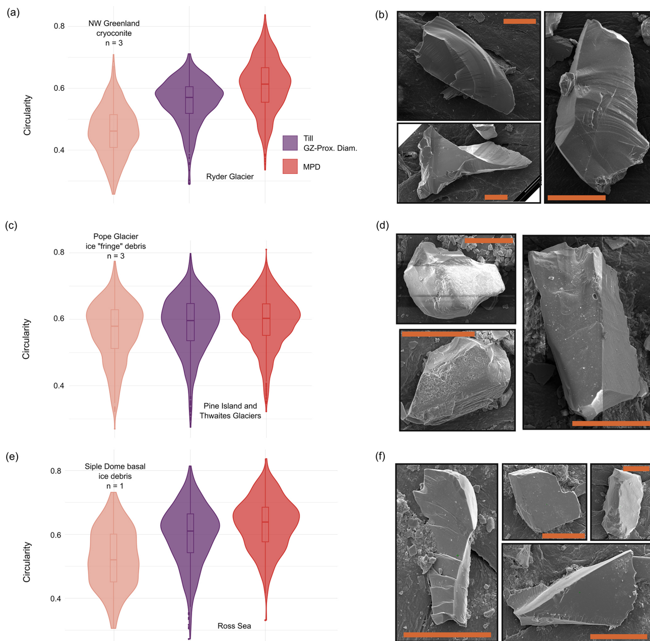
Figure 7. Grain shape evolution. Panels (a), (c), and (e) show grain circularity for grounding-zone proximal diamicton (GZ-Prox. Diam), subglacial till, and meltwater plume deposits in comparison to supra- or englacial reference material from a neighboring glacial catchment. SEM images of (b) supraglacial cryoconite, (d) basal fringe debris, and (f) englacial debris from the base of an ice dome. Note that in (c) the middle violin includes samples from grounding-zone proximal diamicton offshore the Pine Island and Thwaites glaciers, as well as subglacial till samples from Pine Island Glacier (Table A1). Scale bar in (b), (d), and (f) is 20 \mu\text{m} .
