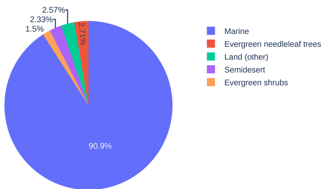
Figure 5. ARMTRAJ-PBL bulk analysis of average surface and vegetation properties overpassed by ECAPE PBL air masses (see the main text).
