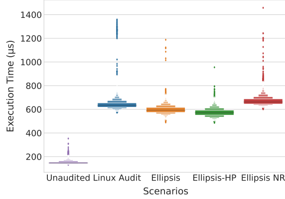
Fig. 9. (§5.6) Comparison of runtime overheads of ArduPilot main loop. The task period and deadline is 2500 \mu s. Ellipsis NR (No Reduction) refers to a forced scenario where each template match fails, leading to no log reduction.
