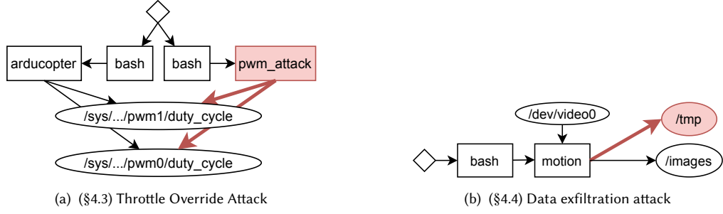
Fig. 4. Attack graphs created using Ellipsis audit logs.
