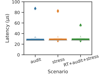
Fig. 12. Latency of a syscall execution with same priority parallel threads. Fig. 13. The overhead of auditing getpid with stress.
