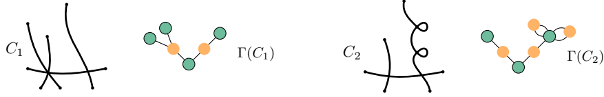
FIGURE 1. Examples of curves and their intersection graphs.
