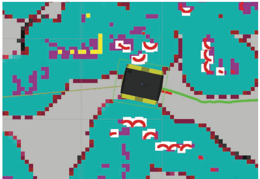
FIGURE 5. Rviz visualization of obstacles in the MPC. White squares: obstacle coordinates sampled from raw lidar scan. Yellow squares: blind spot obstacle coordinates obtained from local_costmap .
