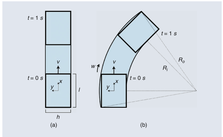
FIGURE 4. (a) and (b) Safety zone illustration for the safety-check layer of LiCS during linear and radial movement.
