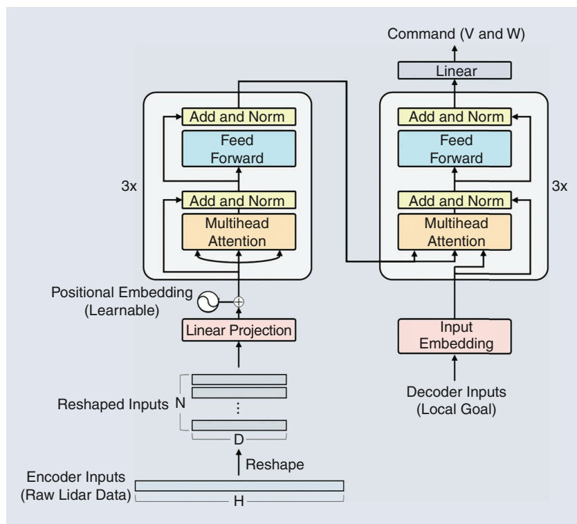
FIGURE 3. Transformer-based neural network used in LiCS.
