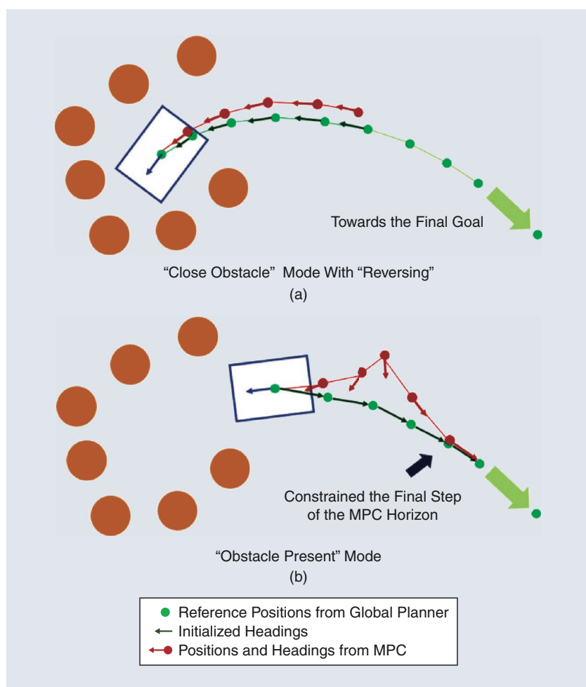
FIGURE 6. Different modes with different initialization and limits. (a) “Close obstacle” with “reversing” mode has the headings pointing away from the goal to allow safe backtracking. (b) “Obstacle present” mode has normal heading initialization and constraints allowing the robot to rotate to the correct heading.
