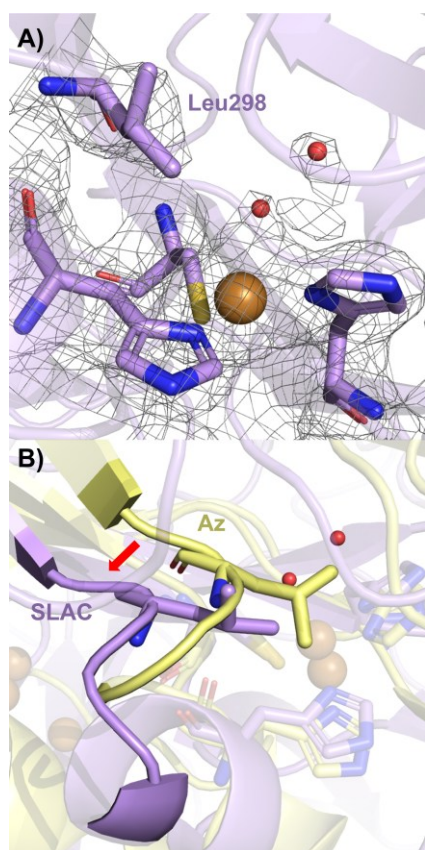
Figure 3. A) Crystal structure of M298L-SLAC (PDB: 9NJI) showing the axial water (red spheres), with a 2F_o - F_c electron density contoured at 1 RMSD; B) Structure alignment between M298L-SLAC (purple, PDB: 9NJI) and N47S/M121L-azurin (yellow, PDB: 3JT2 8 ). The red arrow indicates the shift of the loop that holds the axial leucine. The red spheres indicate the axial water in M298L-SLAC.
