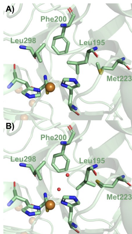
Figure 5. Crystal structure of LF-M298L-SLAC (PDB: 9NJJ) showing the two F195L conformations in subfigure A and B. The axial water is shown in red spheres.
