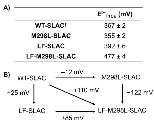
Figure 2. A) E^{\circ'}_{\text{T1Cu}} for mutants involved in this paper. All were measured in 50 mM MOPS, 150 mM NaCl, pH 7 buffer. † Data from ref. 38. B) Relative E^{\circ'}_{\text{T1Cu}} change between each mutant.
