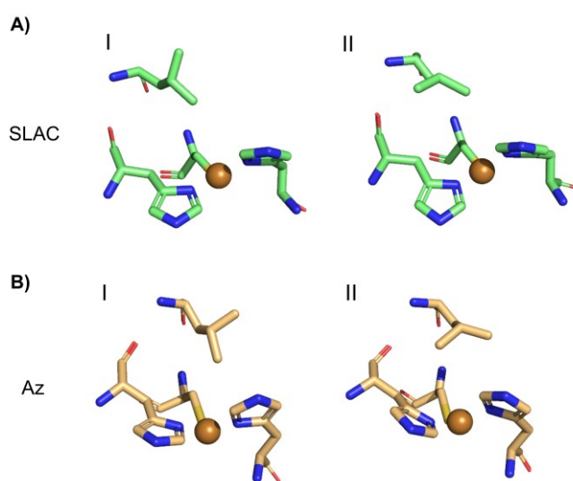
Figure 4. Two conformations (I and II) that the axial leucine can adopt from MD simulation of. A) M298L-SLAC; B) N47S/M121L-Az.
