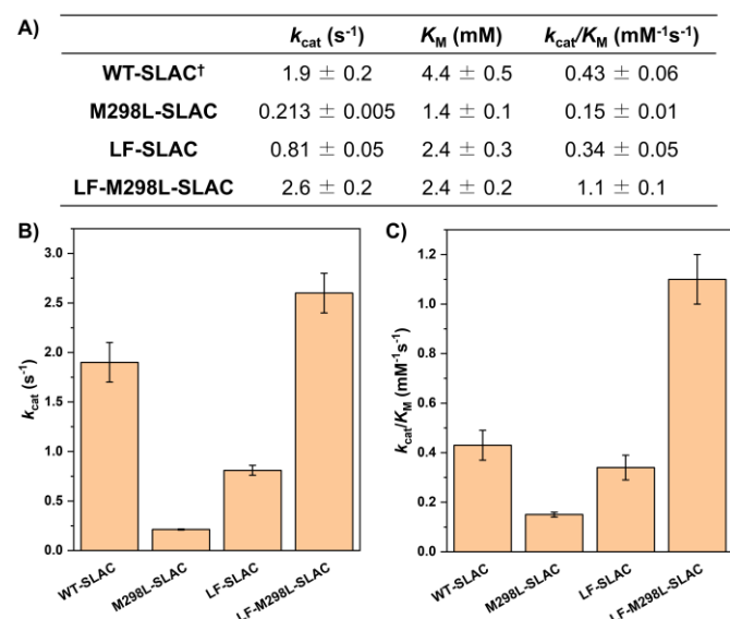
Figure 6. A) Michaelis-Menten parameters for mutants involved in this paper using ABTS as substrate. † Data from ref. 38. (Michaelis-Menten parameters were measured in 50 mM MOPS, 150 mM NaCl, pH 7 at 310 K.) Histogram demonstrating B) k_{\text{cat}} , and C) k_{\text{cat}}/K_{\text{M}} for different mutants.
