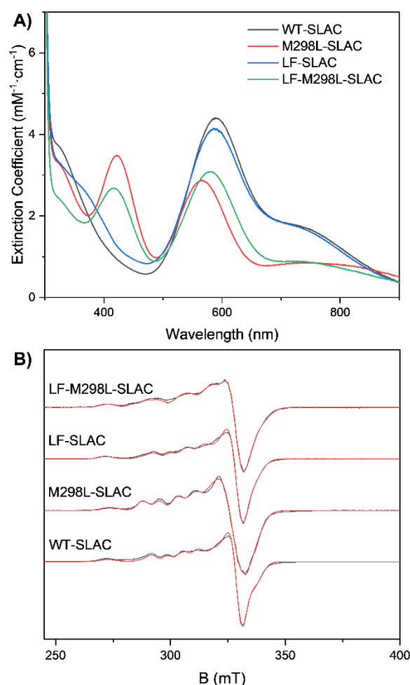
Figure 1. A) Electronic absorption spectrum and B) EPR spectrum (Black: Experimental spectra; Red: Fitted spectra) of SLAC mutants involved in this study. Data for WT-SLAC is replotted from ref. 38 . LF-SLAC stands for F195L/I200F-SLAC.
