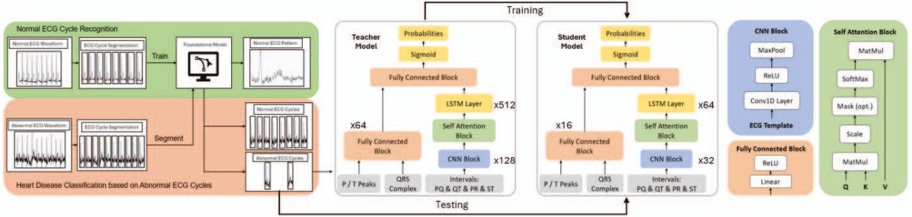
Figure 1: The two-stage framework of the proposed efficient cardiovascular disease detection. Computational overhead is reduced by only conducting analysis on abnormal ECG cycles selected by the lightweight foundation model.
