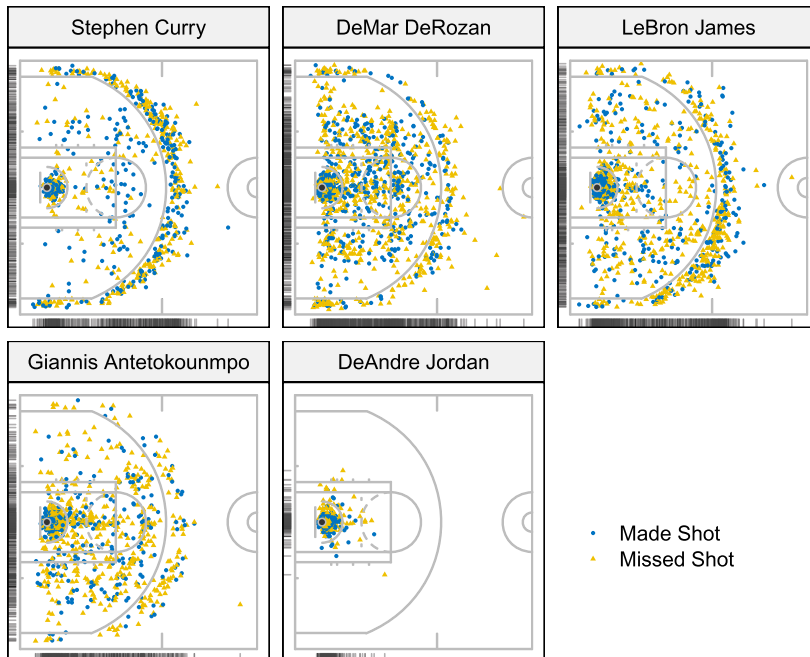
FIG. 1. Field Goal Attempts Data Display. On half court image, each point represents one shot. The marginal distributions of the shot locations are shown on the left and down sides of each plot, respectively. (Players: Stephen Curry, DeMar DeRozan, LeBron James, Giannis Antetokounmpo, DeAndre Jordan).
