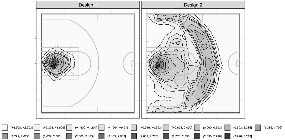
FIG. 2. Contour Plots for Intensity Maps of Two Simulation Designs.
