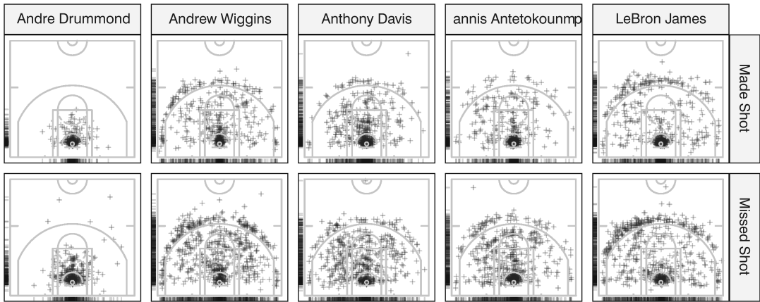
FIG. 6. Top five Players with smallest P -values based on our proposed test framework. Each column indicates the Made pattern (Top) and Missed pattern (Bottom) of the respective player.
