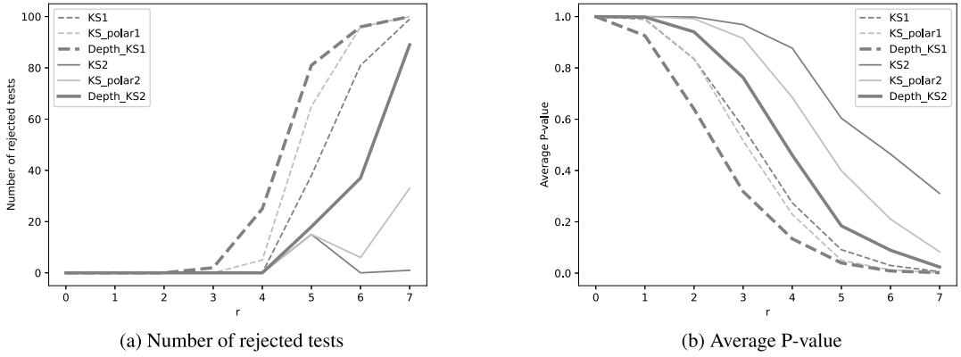
FIG. 3. “KS1” is the two-dimensional KS test on Group 1 (Method 3), “KS-polar1” is the two-dimensional KS test based on polar coordinate for Group 1 (Method 4), and “Depth-KS1” is the proposed test scheme for Group 1. Similar notation applies to Group 2: (a). Plot of number of rejected tests ( \alpha = 0.05 ) for Group 1 (dash line) and Group 2 (solid line) based on the proposed test scheme, KS test, and KS test on polar coordinate. (b). Corresponding average P -value plot.
