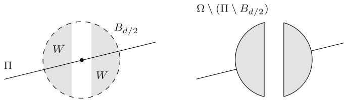
Fig. 3. The obstacle W (depicted in grey) is obtained by removing a cylinder C_r^{en+1} from a ball B_{d/2} with d/2 > r . In this way d = \text{diam}(W) and B_{d/2} is the only ball such that (1.17) can hold. Hyperplanes \Pi satisfying (1.17) are exactly those passing through the center of B_{d/2} , and intersecting W on a (n-1) -dimensional sphere of radius d/2 . For every such \Pi , \Omega \setminus (\Pi \setminus B_{d/2}) has exactly one unbounded connected component, and (1.18) does not hold
