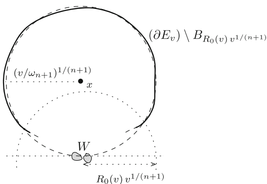
Fig. 1. Quantitative isoperimetry gives no information on how W affects \psi_W(v) for v large
