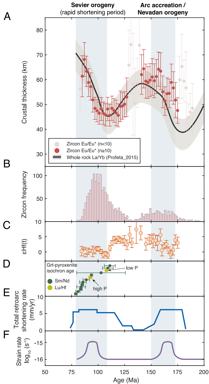
Fig. 3. A. Crustal thickness evolution of the Sierra Nevada batholith reconstructed using \text{Eu}/\text{Eu}^* in detrital zircon. The data are plotted as binned averages (bin size = 2 Myr) and 2 SE errors. For each bin, we removed 10 % of the data with the highest values and 10 % with the lowest values to minimize the influence of outliers. The dark curve bracketed by a gray band shows the average crustal thickness, with 2 SE margins, calculated from \text{La}/\text{Yb} ratio of felsic rocks within the Sierra Nevada batholith (Profeta et al., 2015). B. Age distribution of detrital zircon analyzed in this study. C. Evolution of Hf isotopes of the Sierra Nevada batholith compiled by Cao et al. (2022). D. Mineral Sm/Nd and Lu/Hf isochron ages of garnet pyroxenite cumulates in the Sierra Nevada region (Chin et al., 2015; Ducea and Saleeby, 1998b). E. Total retro-arc shortening rate (Yonkee and Weil, 2015). F. Intra-arc strain rate estimated by Cao et al. (2015).
