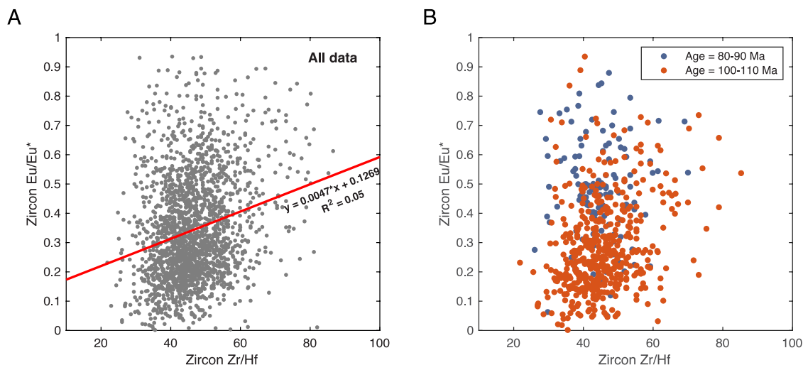
Fig. 5. Zircon Eu/Eu*-Zr/Hf relationships in our Sierran Nevada detrital zircon dataset. A. All data are plotted. B. Two subsets of data with ages of 80–90 Ma and 100–110 Ma are plotted.
