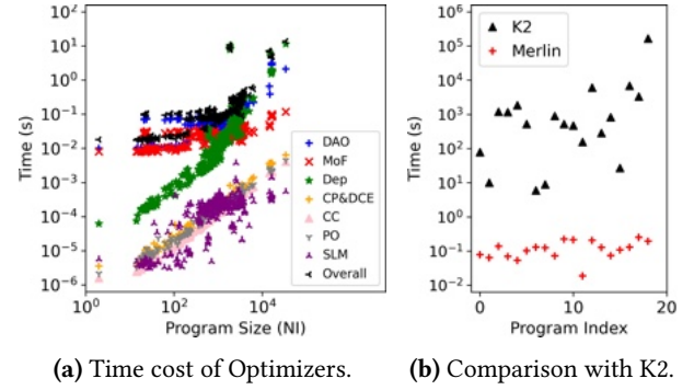
(a) Time cost of Optimizers. (b) Comparison with K2. Figure 13. Compilation Costs of MERLIN. Labels are Data Alignment Optimization (DAO), Macro-op Fusion (MoF), Dependency analysis (Dep), Code Compaction (CC), Peephole Optimization (PO), and Superword Level Merging (SLM).
