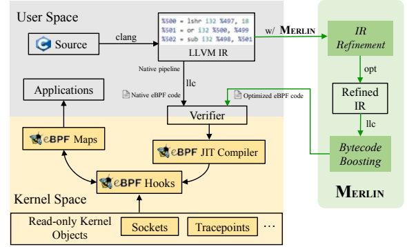
Figure 1. eBPF Workflow
