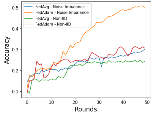
Figure 1: Testing accuracy vs. federation rounds under high noise and class imbalance for 16 clients.
