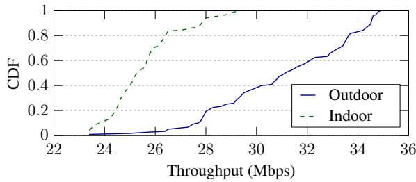
Fig. 7: UDP DL throughput for outdoor and indoor settings.
