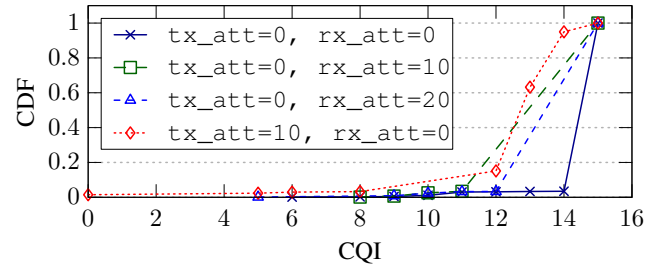
Fig. 6: CQI variation for different attenuation levels.
