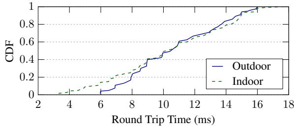
Fig. 8: Round-trip time for outdoor and indoor settings.
