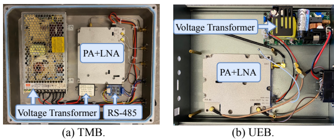
Fig. 3: Internal view of TMB and UEB.
