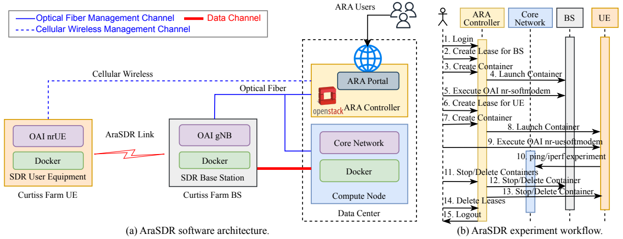
Fig. 4: AraSDR software architecture for the OAI experiment in Curtiss Farm.
