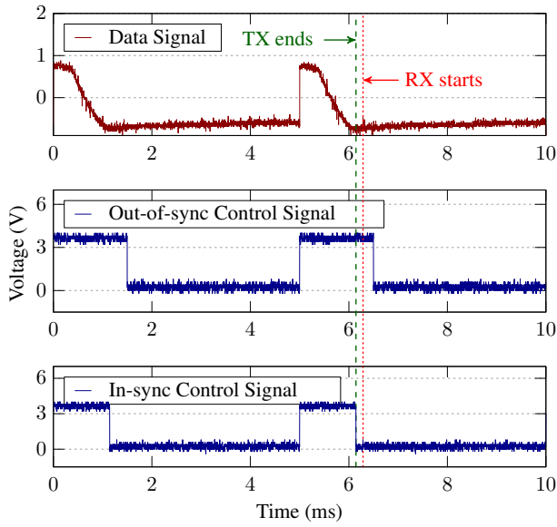
Fig. 5: GPIO synchronization at UEB, with each time slot being 0.5 ms.
