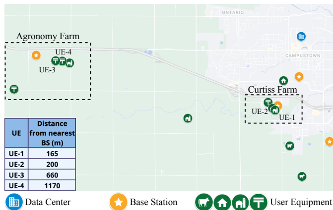
Fig. 1: AraSDR Phase-1 deployment map. The table shows the distance of UEs from the nearest BS. The dashed-rectangles show the experiment location.
