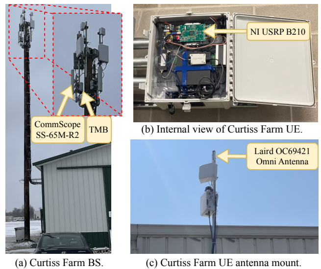
Fig. 2: AraSDR BS and UE deployment at Curtiss Farm.
