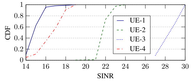
Fig. 9: SINR variation for different UE locations.
