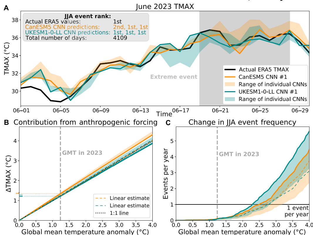
Fig. 2. Machine learning-based extreme event attribution for southcentral North America. (A) Daily TMAX predicted by CNNs during June 2023 (gold/green). Results for CNNs trained on CanESM5 simulations are shown in gold, and results for CNNs trained on UKESM1-0-LL simulations are shown in green. Solid lines show results for one individual CNN, and shading reveals the range of CNN predictions across three CNNs each trained with a different random seed. Actual TMAX values from the European Center for Medium-Range Weather Forecasting Reanalysis fifth generation historical reanalysis (ERA5) are also shown (black). (Gray box) Comparison between the event ranking in the distribution of actual ERA5 TMAX data and the event ranking in the distribution of CNN predictions (for each CNN used in this analysis). Event rank is calculated by counting the number of distinct 10-day periods in June to August (JJA) 1979 to 2023 in which the 10-day average TMAX surpasses the average TMAX during the 19 to 28 June 2023 event. (B) Change in the mean counterfactual TMAX prediction during the 19 to 28 June 2023 event as a function of the GMT input value, for values ranging between +0.0° and +4.0°C relative to the 1850 to 1900 baseline period (i.e., the GMT anomaly). (C) The number of 10-day periods hotter than the June 2023 event as a function of the GMT anomaly calculated using the counterfactual CNN predictions from the ERA5 input maps during the JJA 1979 to 2023 period. Dashed lines in (B) and (C) show the estimated change in event magnitude and frequency predicted by a linear extrapolation of the ERA5 TMAX values to different levels of GMT according to the calendar-day linear trend in TMAX (calculated with respect to GMT) from the CanESM5 and UKESM1-0-LL realizations.
