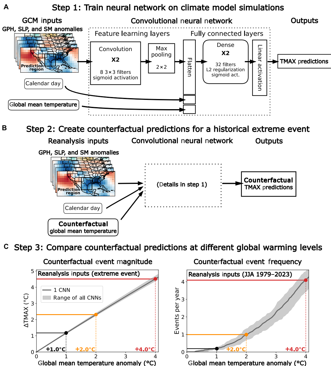
Fig. 1. Schematic of machine learning–based approach for extreme event attribution. (A) A CNN is trained to predict the daily TMAX over the prediction region (black box) using the following inputs: the calendar day, the annual GMT, and two-dimensional calendar-day anomaly maps of SLP, SM, and GPH at 700, 500, and 250 mbar. Three CNNs are trained on data from GCM simulations for the 1850 to 2100 period. See Materials and Methods for details of the CNN architecture and training process. (B) The trained CNNs are used to predict TMAX for a historical extreme event using the input variables from a historical reanalysis. Then, counterfactual TMAX predictions for this extreme event are obtained by letting the GMT input vary between +0.0^{\circ} and +4.0^{\circ} C relative to the 1850 to 1900 baseline period (i.e., the GMT anomaly). (C) (Left) Change in the counterfactual CNN TMAX prediction as a function of the GMT anomaly calculated using the reanalysis input maps from the historical extreme event. (Right) The number of extreme events [hotter than the event from (B)] as a function of the GMT anomaly calculated using the counterfactual CNN predictions from the reanalysis input maps during the June to August 1979 to 2023 period. Shown are the results for one individual CNN (dark gray line) and the range of results from three CNNs (gray shading) each trained with a different random seed.
