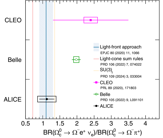
FIG. 4. Comparison of \text{BR}(\Omega_c^0 \rightarrow \Omega^- e^+ \nu_e) / \text{BR}(\Omega_c^0 \rightarrow \Omega^- \pi^+) between experiments and theoretical calculations [26,31–33,36].
