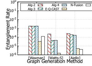
Fig. 5. Entanglement rate v.s. Network topology.
