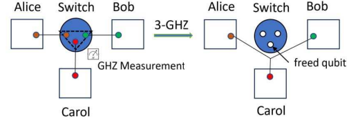
Fig. 2. 3-fusion: it fuses three quantum links and entangles three qubits.
