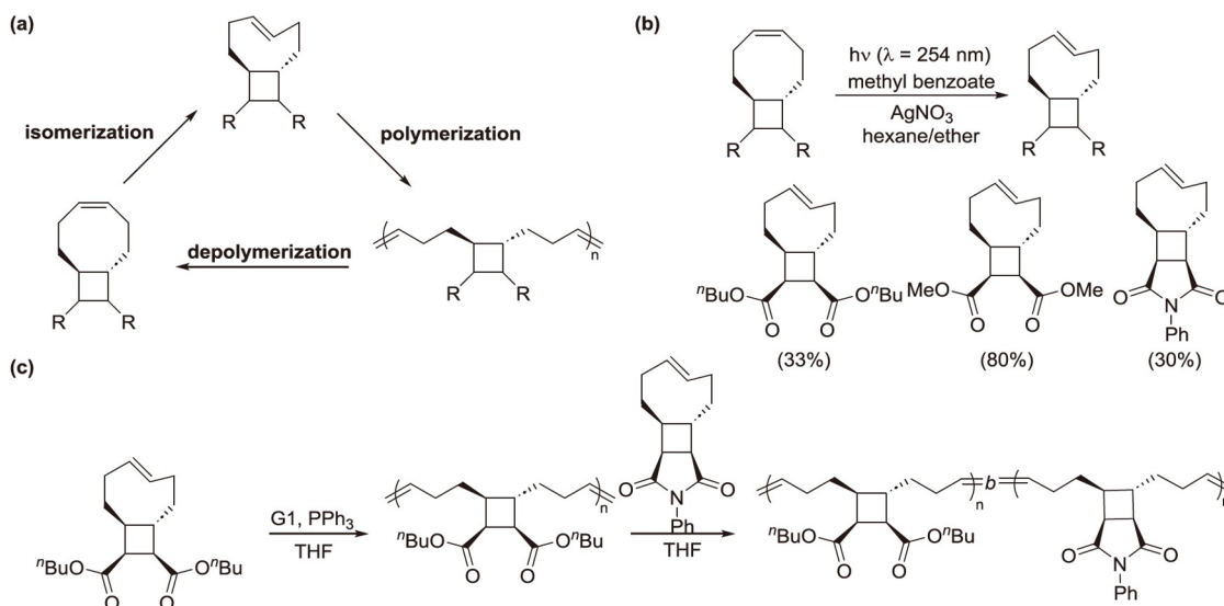
Figure 32 Trans-alkene tCBCO monomers used in making depolymerizable polymers. Reproduced from Ref. [224] with permission. Copyright 2021 Wiley-VCH GmbH. (a) Schematic showing conversion of cis-alkene-tCBCO monomer into its trans-alkene isomer, polymerization of the trans-alkene monomer, and depolymerization of the resulting polymer back to the cis-alkene tCBCO monomer. (b) Photochemical isomerization of the cis-alkene tCBCO monomers into their trans-alkene isomers; the yield for each product is shown in parentheses. (c) Synthesis of homopolymer and block copolymer using the trans-alkene tCBCO monomers.
