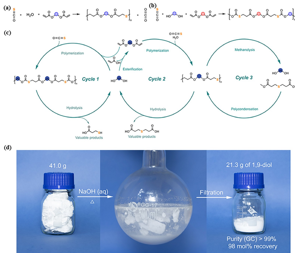
Figure 20 (a) Synthesis of polymers with in-chain ester and thioether groups from polymerization of COS, H 2 O, and diacrylates. (b) Synthesis of polymers with in-chain ester and thiocarbonate groups from polymerization of COS, diols, and diacrylates. (c) Schematic diagram of the chemical recycling of the polymers: Cycle 1 shows the cycle of the second system; Cycles 2 and 3 show the cycle of the first system. (d) Chemical recyclability of obtained polymers. Reproduced from Ref. [113] with permission. Copyright 2023 Wiley-VCH GmbH (color online).
