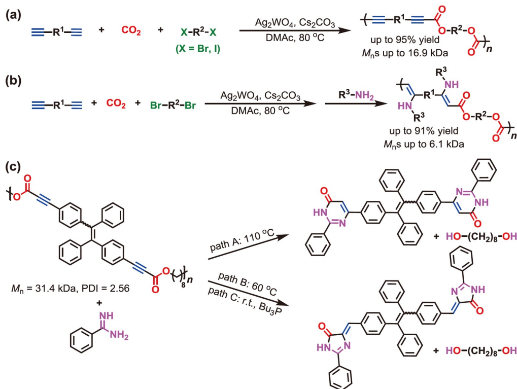
Figure 26 CO 2 -based MCP for the synthesis of (a) poly(alkynoate)s and (b) poly(aminoacrylate)s. (c) The degradation of CO 2 -based poly(alkynoate)s (path A: benzamidine, 110 °C; path B: benzamidine, 60 °C; path C: benzamidine, r.t., \text{Bu}_3\text{P} ) (color online).
