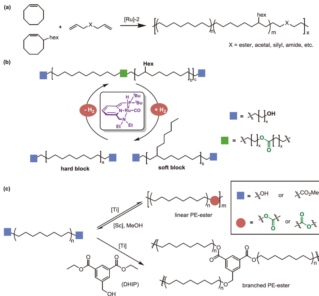
Figure 24 (a–c) The synthesis of chemically recyclable polyolefin-like polymers with telechelic macromonomers derived from ROMP of cyclooctene monomers. Reproduced with adaptation from Ref. [175] with permission. Copyright 2022 Springer Nature (a); Reproduced from Ref. [176] with permission. Copyright 2023 American Association for the Advancement of Science (b); Reproduced with adaptation from Ref. [177] with permission. Copyright 2024 American Chemical Society (c) (color online).
