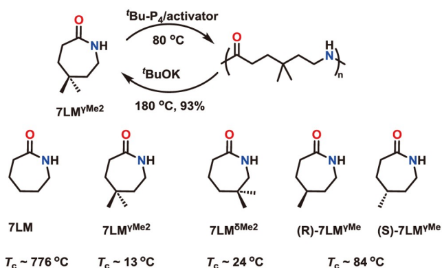
Figure 16 Polymerization and depolymerization of gem -dimethyl substitution \varepsilon -caprolactam (color online).
