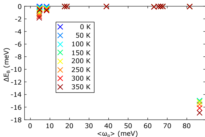
Fig. 5. Contribution of different phonon modes to the exciton binding energy shift of GaN due to phonon screening, as a function of temperature. Here, \langle\omega_q\rangle denotes the average frequency of a particular phonon branch across the studied patch of the Brillouin zone.
