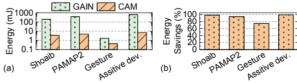
Figure 4: a) Comparison of energy consumption for GAIN and CAM. The y-axis is shown in log scale to represent the large range of values. b) Energy savings achieved by CAM compared to GAIN.
