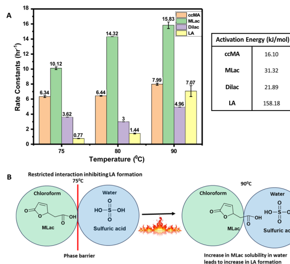
Fig. 7 (A) Rate constants (k), equilibrium constants (K) and activation energies for the reaction of cis,cis -muconic acid (ccMA) to levulinic acid (LA). (B) Illustrative figure depicting the phase barrier of chloroform and water inhibiting the LA formation at 75 °C and surmounting the barrier at 90 °C.
