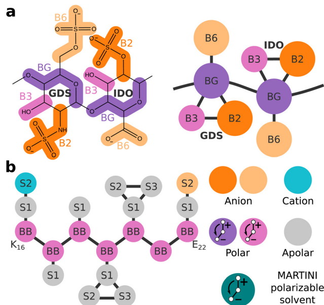
Fig. 1 (a) Mapping of the CG heparin model. (b) Schematic representation of the CG A \beta_{16-22} fragment K 16 LVFFAE 22 (left). A key for the bead types, and a schematic depiction of the CG MARTINI polarizable solvent model (right). The anionic and cationic dummy particles of any polar bead X would be named X m and X p , respectively.
