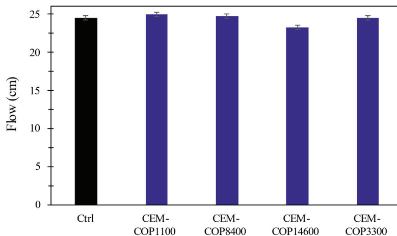
Figure 8. Flow of samples with copolymer concentration of 0.25% w/w cement at a W/C of 0.4.
