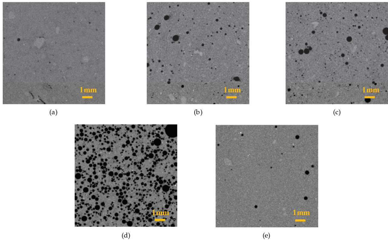
Figure 9. Micro-CT cross-sections of samples at mid-length with 0.25% of copolymer as air-entraining agents. (a) Ctrl. (b) CEM-COP1100. (c) CEM-COP8400. (d) CEM-COP14600. (e) CEM-COP3300.
