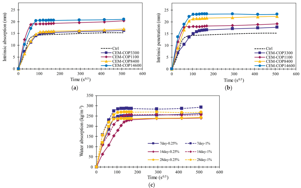
Figure 11. Gravimetric water penetration and absorption at 28 days between different copolymer samples (a) with 0.25% concentration, (b) with 1% concentration, and (c) CEM-COP14600 at different ages and concentrations.
