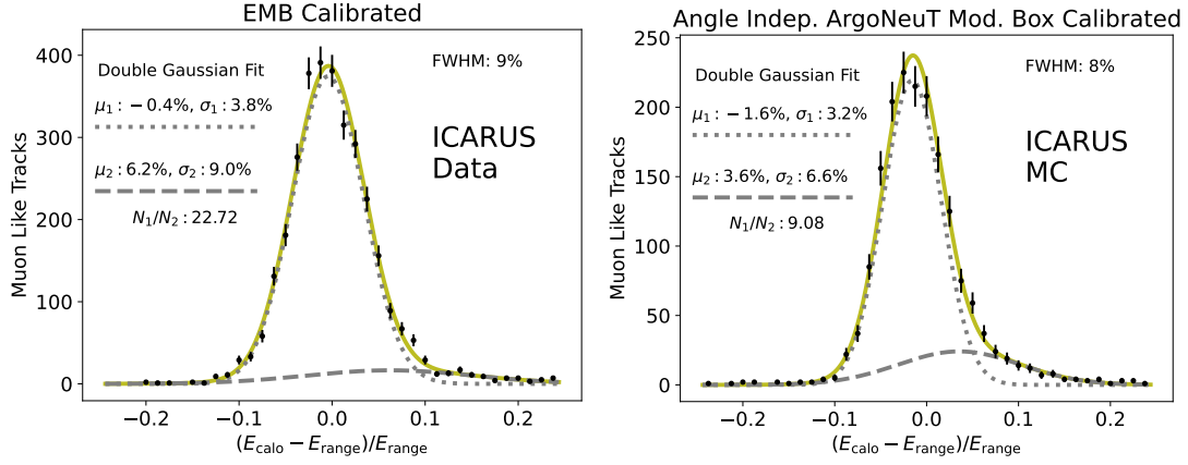
Figure 13. Comparison of calorimetric energy ( E_{\text{calor}} ) and range energy ( E_{\text{range}} ) reconstruction for selected muons in ICARUS data (left) and Monte Carlo simulation (right). The EMB-based calibration is applied in data. The Monte Carlo simulation applies the ArgoNeuT angle-independent modified box model for both simulating recombination and correcting for it. The calorimetric energy applies the “Q-tip” energy reconstruction and includes a correction for missing hits along the track. The data points are fit to a sum of two Gaussian distributions with centers ( \mu_1, \mu_2 ) and standard deviations ( \sigma_1, \sigma_2 ). The ratio of the amplitudes of the Gaussian distributions is quoted as N_1/N_2 .
