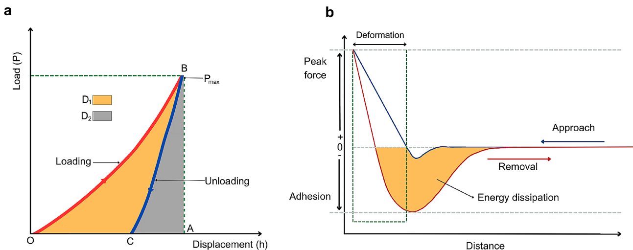
Fig. 1 Representation of work done in (a) the nanoindentation and (b) AFM processes (Adapted from [18, 23])
