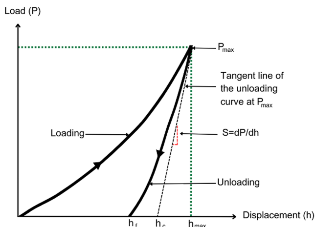
Fig. 4 Representation of loading and unloading curve during the nanoindentation process (Adapted from [10, 48])
