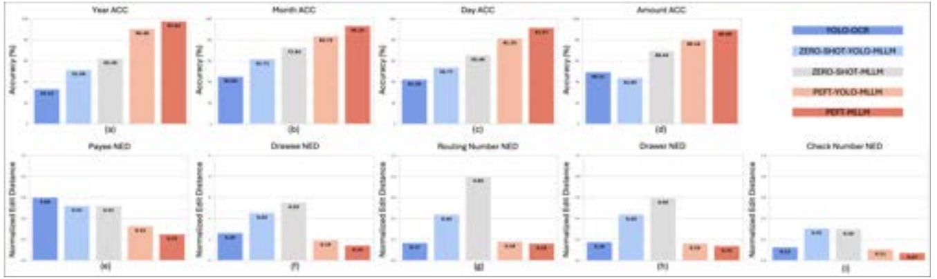
Figure 3: Benchmark results of the experiment
