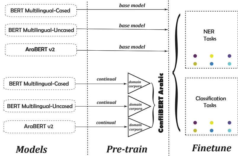
Figure 1: Workflow of our ConflBERT-Arabic framework.
