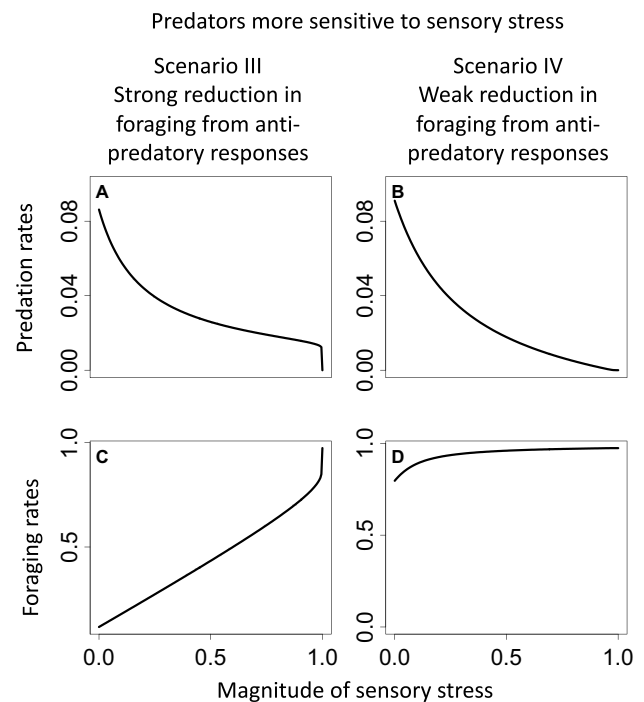
Fig. 5 The predation ( w ) and foraging ( v ) rates of the predator and prey, respectively, for scenario III I ( n=25 , m=2 ) and IV ( n=25 , m=0.2 ) across a range of values for sensory stress s . Total predation rates decline with sensory stress in both scenarios (panels A , B ) since predators are more sensitive to sensory stress with a corresponding increase in foraging rates by prey (panels C , D )
