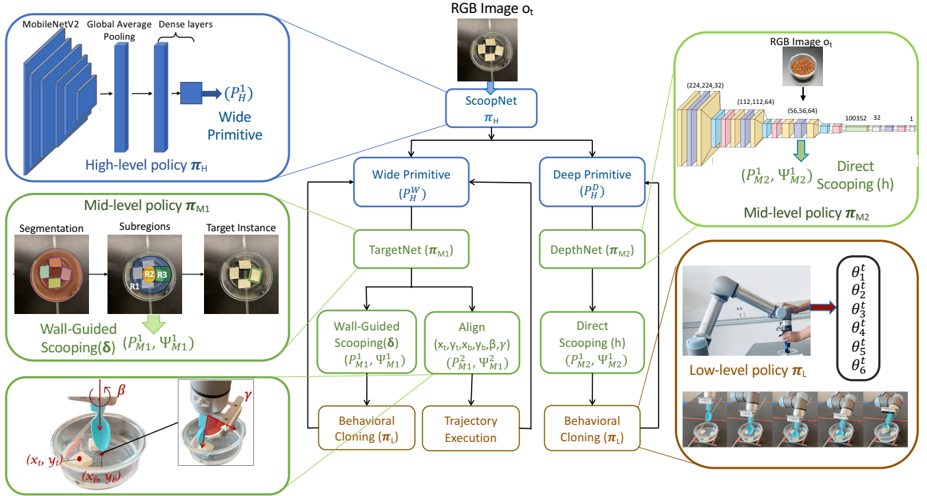
Fig. 2: System Architecture of LAVA, employs a high level policy(blue) \pi_H to select amongst discrete high level primitives P_H^k , which further gets refined by mid-level policy (green) \pi_M to select amongst mid-level primitives P_M^k , low-level vision parametrized policy \pi_L (brown) executes trajectory learned from Behavioral cloning for long-horizon food acquisition.
