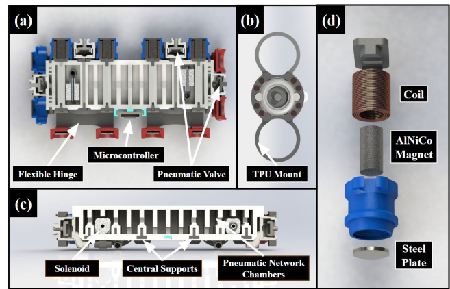
Figure 2. a) Top-down cross-sectional view of the actuator. b) PAC connector and soft mounting TPU component. c) Side, cross-sectional view of actuator. d) Exploded view of RMCs showing the plastic casing, AlNiCo magnet, steel plate, and wire coil.
