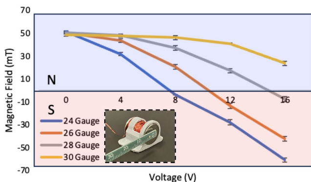
Figure 6. Reversible magnet with coil testing results. The graph represents the magnetic field of four trials with varying wire diameters and voltages. Each test was repeated two times. The magnetic field strength was measured at the tip of the magnet, as seen in the embedded image.
