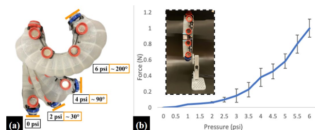
Figure 5. a) Visualization of the correlation between air pressure and angle of actuation. b) Blocked force data of a single actuator, showing the relationship between air pressure and produced force. Embedded image shows setup for recording blocked force data.
