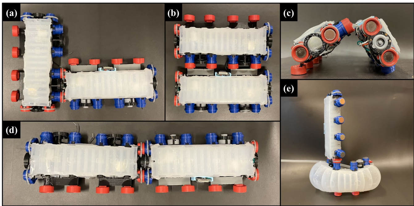
Figure 7. Various reconfiguration combinations of modular actuators assembled manually for demonstration purposes. a) End-to-side type connection. Side-to-side connection in b) planar form and c) spatial form with flexible hinges bent. d) End-to-end connection. e) End-to-side connection in spatial form.
