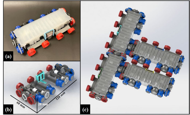
Figure 1. a) Elemental modular actuator. b) Dimensioned CAD view of the modular actuator with the soft silicone component removed, showing internal support structure. c) Examples of inter-unit connections.
