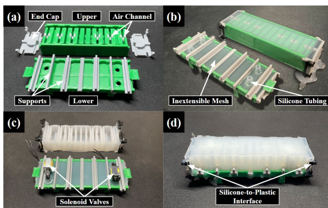
Figure 4. Molding of the pneumatic actuator. a) 3D printed mold pieces for fabricating the actuator. b) Pouring silicone rubber into the molds to create upper and lower sections of the pneumatic network. c) Placement of solenoids with attached 3D printed fittings through silicone tubes of bottom mold. d) Final step of molding process, where top and bottom sections are glued together with additional silicone rubber.
