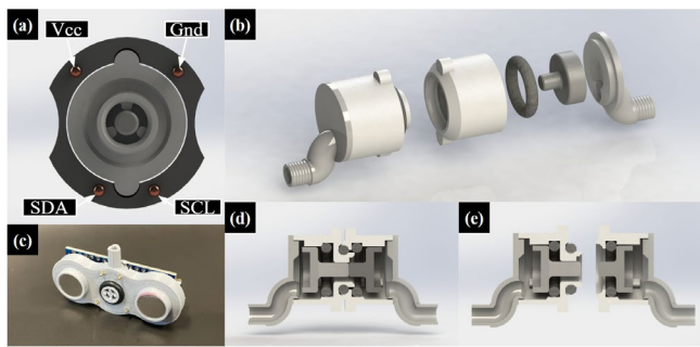
Figure 3. PAC connector. a) Front view with indicated spring-loaded pogo pins for electrical connections. b) Exploded view of a PAC connector showing valves, housing, and O-ring. c) Input module in a housing with a master control board for communication and PAC connection for main power and air input (air supply tubes and wires not shown). d) Open and e) closed state of a custom, miniature pneumatic valve.
