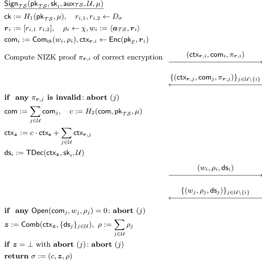
Fig. 7. Actively secure 2-round t -out-of- n threshold signature protocol for signer \mathcal{S}_i .
