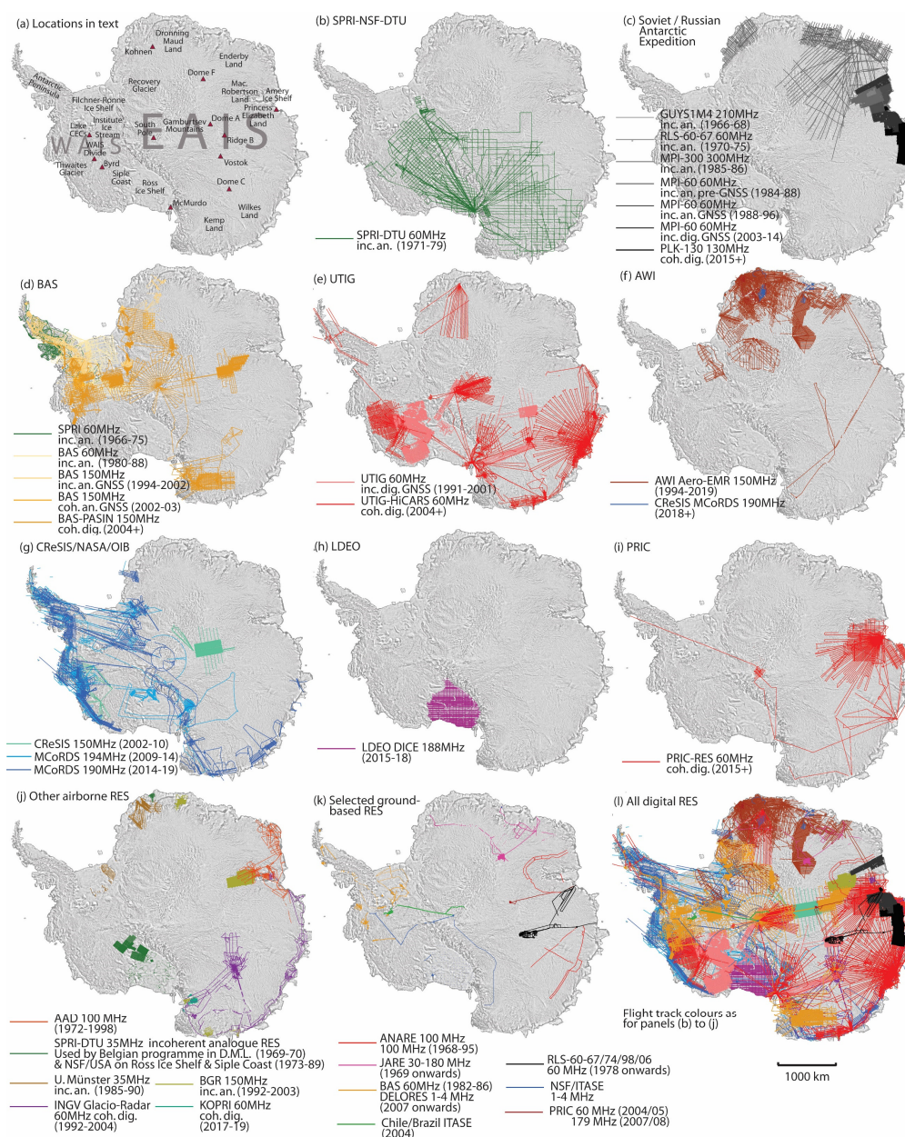
Figure 3. (a) Reference map of main Antarctic locations mentioned in this review. (b) to (j) Airborne RES coverage by data provider as discussed through Sect 3.1 to 3.9. Each legend outlines basic details of the provider's RES system by system-name, typical centre frequency, whether the system was incoherent (inc.) or coherent (coh.), whether the acquisition was analogue (an.) or digital (dig.), whether flight navigation used GNSS (assumed not for data collection before 1990), and the date ranges over which a system was used. (k) Coverage of long-range ground-based RES data across Antarctica with potential for extraction of deep internal-reflecting horizons. (l) Combined coverage of all digital RES datasets across Antarctica with potential for contributing to AntArchitecture .
