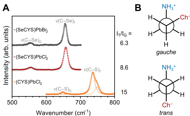
Figure 2. (A) The trans and gauche \nu(\text{C–Ch}) Raman modes ( \text{Ch}=\text{S}, \text{Se} ) in the organochalcogenide-halide perovskites. The I_T/I_G value gives the ratio between trans and gauche conformers using integrated peak intensities. Open circles: experimental Raman data; solid line: total fit; dashed line: individual fit in \nu(\text{C–S})_T for (CYS)PbCl 2 . (B) Newman projection of the zwitterionic ligand with two possible rotamers ( trans and gauche ).
