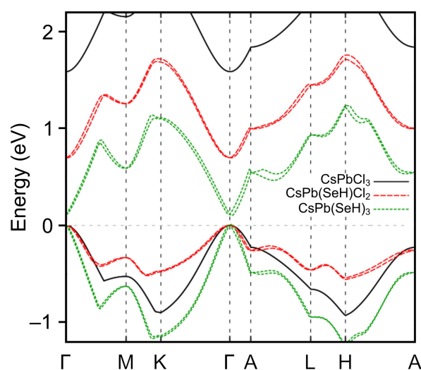
Figure 5. Comparison of the band edges for the hypothetical CsPbCl 3 , trans -CsPb(SeH)Cl 2 , and CsPb(SeH) 3 all in the R-3c space group. The valence band maxima have been arbitrarily aligned, for ease of comparison.
