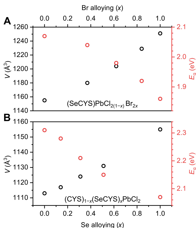
Figure 6. (A) Dependence of the unit-cell volumes ( V ) and band gaps ( E_g ) on the alloying fraction of Br in (\text{SeCYS})\text{PbCl}_{2(1-x)}\text{Br}_{2x} . (B) Dependence of the unit-cell volumes ( V ) and band gaps ( E_g ) on the alloying fraction of SeCYS in (\text{CYS})_{1-x}(\text{SeCYS})_x\text{PbCl}_2 . Unit-cell volumes were extracted by Le Bail refinements. Band gaps were extracted by Tauc plots.
