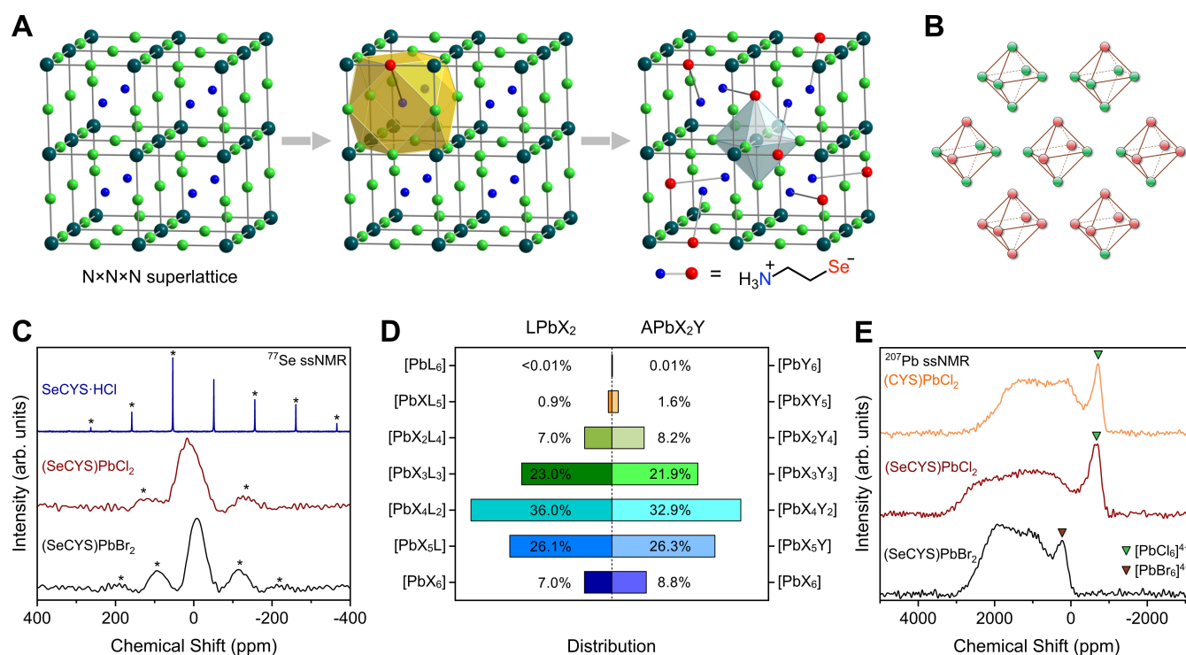
Figure 3. (A) Stepwise illustration of the algorithm used to simulate the random distribution of the organochalcogenide ligand in \text{LPbX}_2 ( \text{L}=\text{CYS} , \text{SeCYS} , \text{X}=\text{Cl} , Br). Step 1: Construct a 200\times200\times200 superlattice of the prototypical perovskite \text{APbX}_3 . Dark turquoise, light green, blue spheres represent Pb, halide, and \text{A}^+ -site cations, respectively. Step 2: For each \text{A}^+ site, find the closest 12 halides (shown in the yellow truncated cube) and randomly choose one to be chalcogenide (red sphere). The connection between the \text{A}^+ site and the chalcogenide stands for a zwitterionic organochalcogenide ligand. Step 3: After repeating step B for all \text{A}^+ sites, find the coordination environments for the Pb centers (shown in the light blue octahedron). (B) The seven distinct coordination environments of Pb octahedra (not distinguishing between cis/trans isomers). The green and red spheres represent the halide and ligand ( \text{L}=\text{SeCYS} , \text{CYS} ), respectively. (C) ^{77}\text{Se} ssNMR spectra of \text{SeCYS-HCl} , (\text{SeCYS})\text{PbCl}_2 , and (\text{SeCYS})\text{PbBr}_2 with a magic-angle spinning (MAS) frequency of 10 kHz at 11.7 T. The asterisks (*) indicate spinning sidebands (identified by varying MAS frequencies, see Figure S16). (D) Comparison of distributions of different Pb coordination spheres, between the fully disordered \text{LPbX}_2 perovskite (left) and the mixed-halide \text{APbX}_2\text{Y} perovskite (right) ( \text{A}=\text{monocation} , \text{L}=\text{zwitterion} , \text{X} and \text{Y} are different halides). (E) ^{207}\text{Pb} ssNMR spectra (without spinning) of (\text{CYS})\text{PbCl}_2 , (\text{SeCYS})\text{PbCl}_2 , and (\text{SeCYS})\text{PbBr}_2 , acquired at 11.7 T. The triangles indicate the peaks assigned to [\text{PbX}_6]^{4-} .
