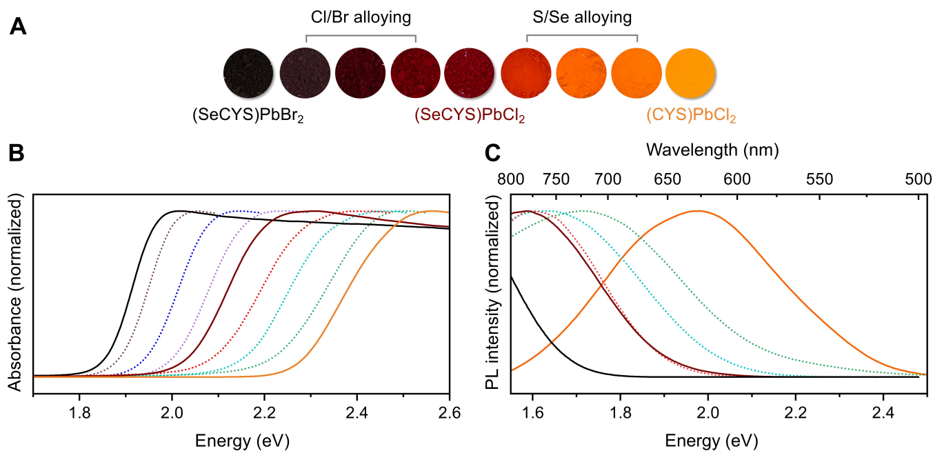
Figure 7. (A) Photographs and (B) diffuse reflectance spectra of powders of (from left to right): (\text{SeCYS})\text{PbBr}_2 (black line), (\text{SeCYS})\text{PbCl}_{2(1-x)}\text{Br}_{2x} (solution-state synthesis; dotted lines), (\text{SeCYS})\text{PbCl}_2 (dark red line), (\text{CYS})_{1-x}(\text{SeCYS})_x\text{PbCl}_2 (dotted lines), and (\text{CYS})\text{PbCl}_2 (solid orange line). (C) Photoluminescence (PL) spectra of (\text{SeCYS})\text{PbBr}_2 (black line), (\text{SeCYS})\text{PbCl}_2 (dark red line), (\text{CYS})_{1-x}(\text{SeCYS})_x\text{PbCl}_2 (dotted lines), and (\text{CYS})\text{PbCl}_2 (solid orange line) measured at 80 K. The full emission of (\text{SeCYS})\text{PbBr}_2 lies outside the detector range, so the lower-energy emission tail was collected using an IR detector (Figures S22–S23).
