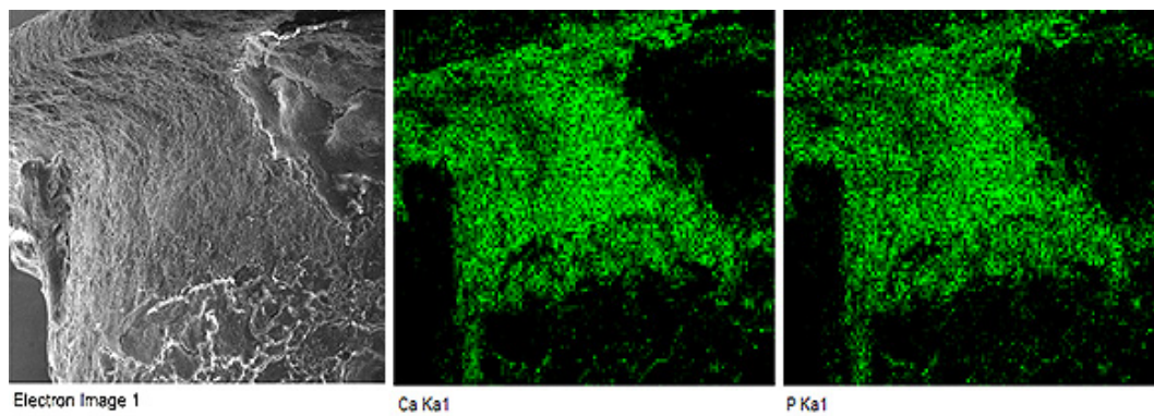
Figure 3. Energy dispersive x-ray spectroscopy areas. The biofilms always tested negative for calcium phosphate (bone mineralization), whereas areas without biofilms tested positive for calcium phosphate (bone mineralization). Ca: Calcium; P: Phosphorus.
