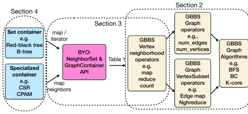
Figure 4: Relationship between BYO framework, graph containers, and graph algorithms (via GBBS).
