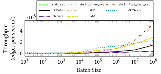
Figure 3: The throughput of inserts for different batch sizes. Of the data structures in this plot, std::set and absl::* are off-the-shelf containers, while the others are optimized. Details on the different graph containers can be found in Section 5.
