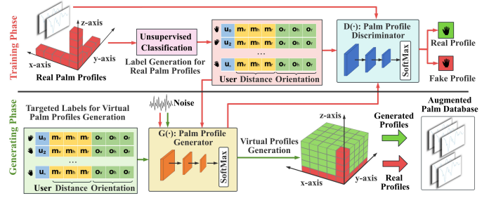
Fig. 6. The process of palm profile augmentation based on cGAN.
