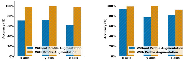
(a) With distance discrepancy (b) With orientation discrepancy Fig. 10. Authentication accuracy before and after involving palm profile augmentation on different palm-device distances and orientations between the enrollment and authentication data.
