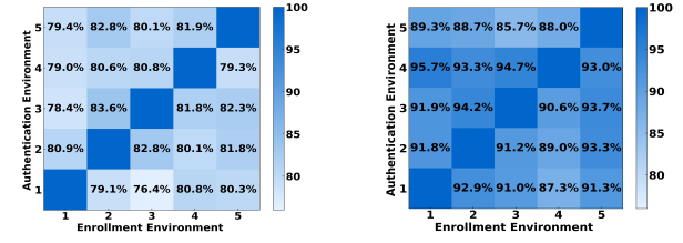
(a) Without adaptation (b) With adaptation Fig. 11. Performance without and with cross-environment adaptation.
