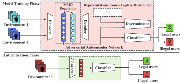
Fig. 7. The cross-environment adaptation module with user classifier.
