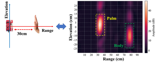
Fig. 4. The Range-Elevation heatmap helps determine the segment of the palm-reflected signals.
