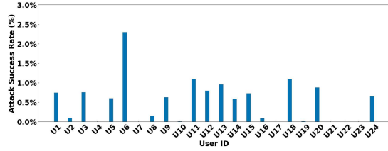
Fig. 12. Attack success rate under impersonation attacks.
