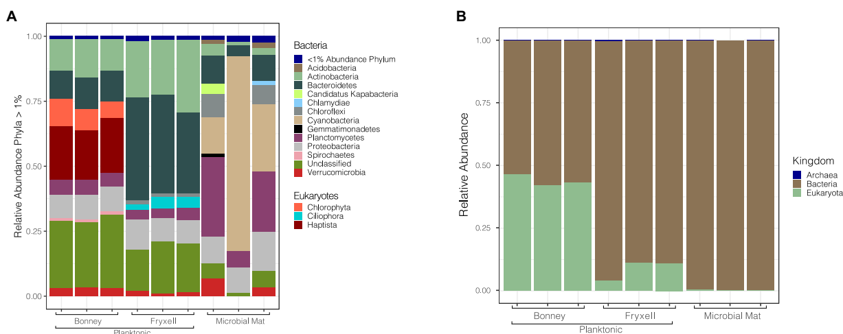
FIGURE 4 Relative abundance of viruses in conjunction with their putative hosts. (A) Predicted viral hosts displayed at the phylum level. Phyla representing less than 1% of the sample are grouped together at the top of the bar plot. (B) Predicted viral hosts at the kingdom level.
