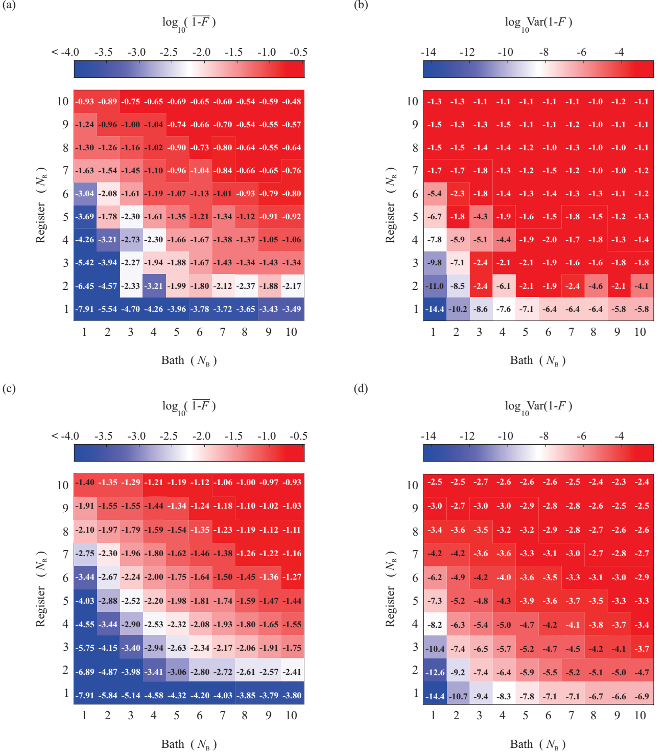
FIG. 4. Gate infidelity ( 1 - F ) versus the size of the bath (unwanted spins) and the size of the register (wanted or target spins) before (a,b) and after (c,d) optimization over single-qubit rotations on the electronic spin. In (a) and (c) we plot the decimal logarithm of the statistical average of infidelity, i.e., \log_{10}(\overline{1 - F}) , while in (b) and (d) we plot the variance of the infidelity on the same logarithmic scale \log_{10} \text{Var}(1 - F) . The numbers in each tile give the value of \log_{10}(\overline{1 - F}) (a,c) and \log_{10} \text{Var}(1 - F) (b,d). In the above simulations, we considered SiC samples with a silicon monovacancy with total spin S = 3/2 , and the electron qubit is defined by (s_0, s_1) = (1/2, 3/2) . The HF values for the ^{13}\text{C} and the ^{29}\text{Si} were drawn from uniform distributions in the intervals 2\pi[10, 200] kHz and 2\pi[0.5, 200] kHz, respectively. The entangling power threshold was set to \epsilon_p^{\text{th}} = 0.85 , the magnetic field is B = 83\text{G} leading to Larmor frequencies (\omega_L^C, \omega_L^{Si}) = 2\pi(88.8797, -70.2595) kHz, and the relative abundance was kept constant for all the cases, i.e., \frac{^{29}\text{Si}}{^{13}\text{C}} = \frac{4.7\%}{1.1\%} = 4.27 . Every data point on the heatmaps was obtained from 200 realizations, and for each trajectory we kept the combination (\tau, N) that resulted in the lowest maximum unwanted one-tangle.
