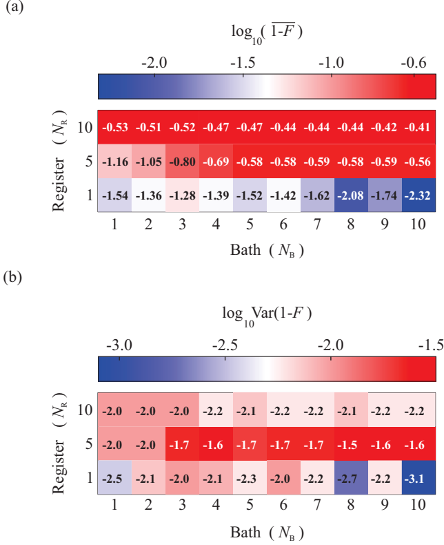
FIG. 8. Effect of changing the sign of a nuclear gyromagnetic ratio. Gate infidelity ( 1 - F ) versus the size of the bath (unwanted spins) and the size of the register (wanted or target spins) upon optimization over single-qubit rotations on the electronic spin. (a) The decimal logarithm of the statistical average of the infidelity, i.e., \log_{10}(\overline{1-F}) . (b) The variance of the infidelity on the same logarithmic scale \log_{10} \text{Var}(1-F) . The number on each tile gives the value of \log_{10}(\overline{1-F}) (a) and \log_{10} \text{Var}(1-F) (b). In the above simulations, we considered fictitious SiC samples with a silicon monovacancy with total spin S = 3/2 , and the electron qubit is defined by (s_0, s_1) = (1/2, 3/2) . The HF values for the ^{13}\text{C} and the ^{29}\text{Si} were drawn from uniform distributions in the intervals 2\pi[10, 200] kHz and 2\pi[0.5, 200] kHz, respectively. The magnetic field was B = 83\text{G} leading to Larmor frequencies (\omega_L^C, \omega_L^{Si}) = 2\pi(88.8797, 70.2595) kHz, and the relative abundance was kept constant for all the cases, i.e., \frac{^{29}\text{Si}}{^{13}\text{C}} = \frac{4.7\%}{1.1\%} = 4.27 . Every data point on the heatmaps was obtained from 100 realizations, and for each trajectory we kept the combination (\tau, N) that resulted in the lowest maximum unwanted one-tangle.
