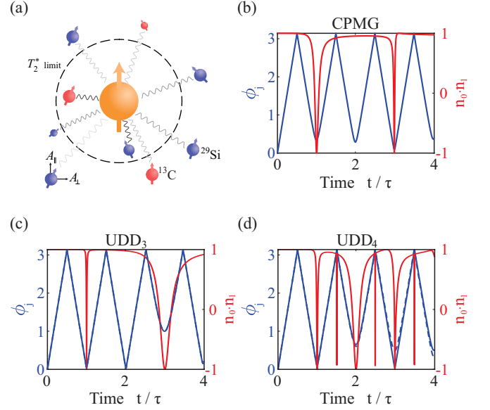
FIG. 1. (a) Schematic depicting a single silicon vacancy coupled to nuclear spins through HF interaction. The spheres denote both nuclear ( 13 C, 29 Si) and electronic spins. Additionally, we illustrate the transition distance between the strongly coupled and weakly coupled regimes, depicted as the T_2^* limit (black dashed line). In (b)-(d) we plot the rotation angles \phi_j (solid and dashed blue lines) and the dot product \mathbf{n}_0 \cdot \mathbf{n}_1 (red color) of nuclear axes as a function of the unit time \tau_k of CPMG, UDD 3 and UDD 4 , respectively. For CPMG and UDD 3 , it holds that \phi_0 = \phi_1 and thus the blue lines (solid and dashed) are on top of each other, while in UDD 4 the two angles are distinguishable. For the nuclear spin, we set (\omega_L, A_{\parallel}, A_{\perp}) = 2\pi \cdot (100, 100, 80) kHz, and the electron's spin projections are (s_0, s_1) = (1/2, 3/2) . The time is normalized to the first order resonance times (\tau_{\text{CPMG}}, \tau_{\text{UDD}_3}, \tau_{\text{UDD}_4}) = (4.6487, 4.6444, 4.6495) \mu\text{s} .
