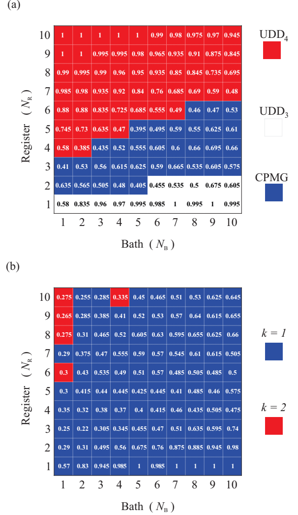
FIG. 7. Best pulse sequence and resonance order versus the size of the bath (unwanted spins) and the size of the register (wanted or target spins). (a) Heatmap depicting the most used (or most probable) DD sequence among CPMG (blue), UDD 3 (white), and UDD 4 (red). (b) Heatmap showing the most used (or most probable) resonance order ( k = 1 blue, k = 2 red) used for \tau_k . The number in each tile refers to the occurrence probability. In the above simulations, we considered SiC samples with a silicon monovacancy with total spin S = 3/2 where the electron qubit is defined by (s_0, s_1) = (1/2, 3/2) . The HF values for the ^{13}\text{C} and ^{29}\text{Si} spins were drawn from uniform distributions in the intervals 2\pi[10, 200] kHz and 2\pi[0.5, 200] kHz, respectively. The entangling power threshold was set to \epsilon_p^{\text{th}} = 0.85 , the magnetic field was B = 83 G leading to Larmor frequencies (\omega_L^C, \omega_L^{\text{Si}}) = 2\pi(88.8797, -70.2595) kHz, and the relative abundance was kept constant for all the cases, i.e., \frac{^{29}\text{Si}}{^{13}\text{C}} = \frac{4.7\%}{1.1\%} = 4.27 . Every data point on the heatmaps was obtained from 200 realizations, and for each trajectory we kept the combination (\tau, N) that resulted in the lowest maximum unwanted one-tangle.
