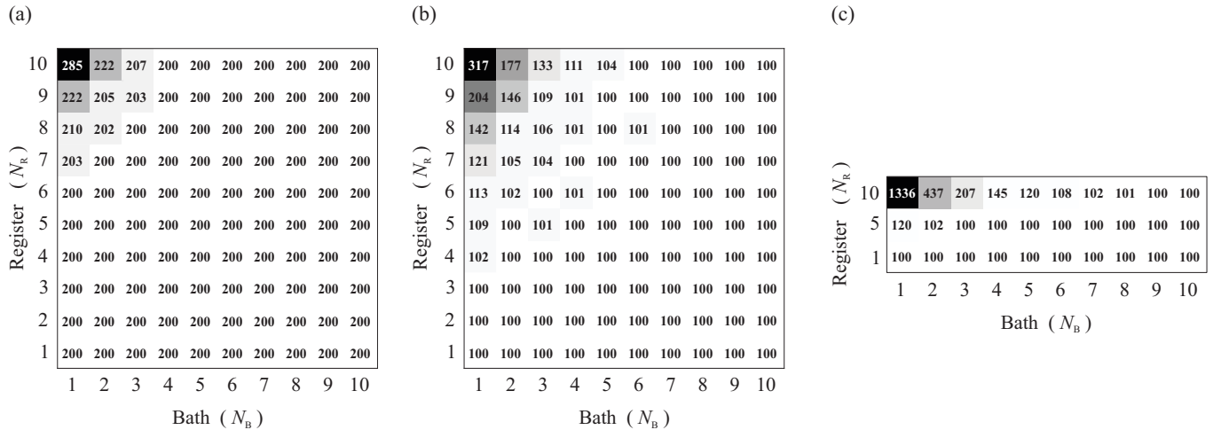
FIG. 9. Total number of realizations simulated to obtain the results presented in the main text. Total number of realizations for (a) a silicon monovacancy defect in SiC, (b) a divacancy, and (c) a monovacancy in the fictitious nuclear spin bath where \gamma_{29\text{Si}} > 0 . The successful realizations for (a), (b), and (c) were 200, 100, and 100, respectively.
