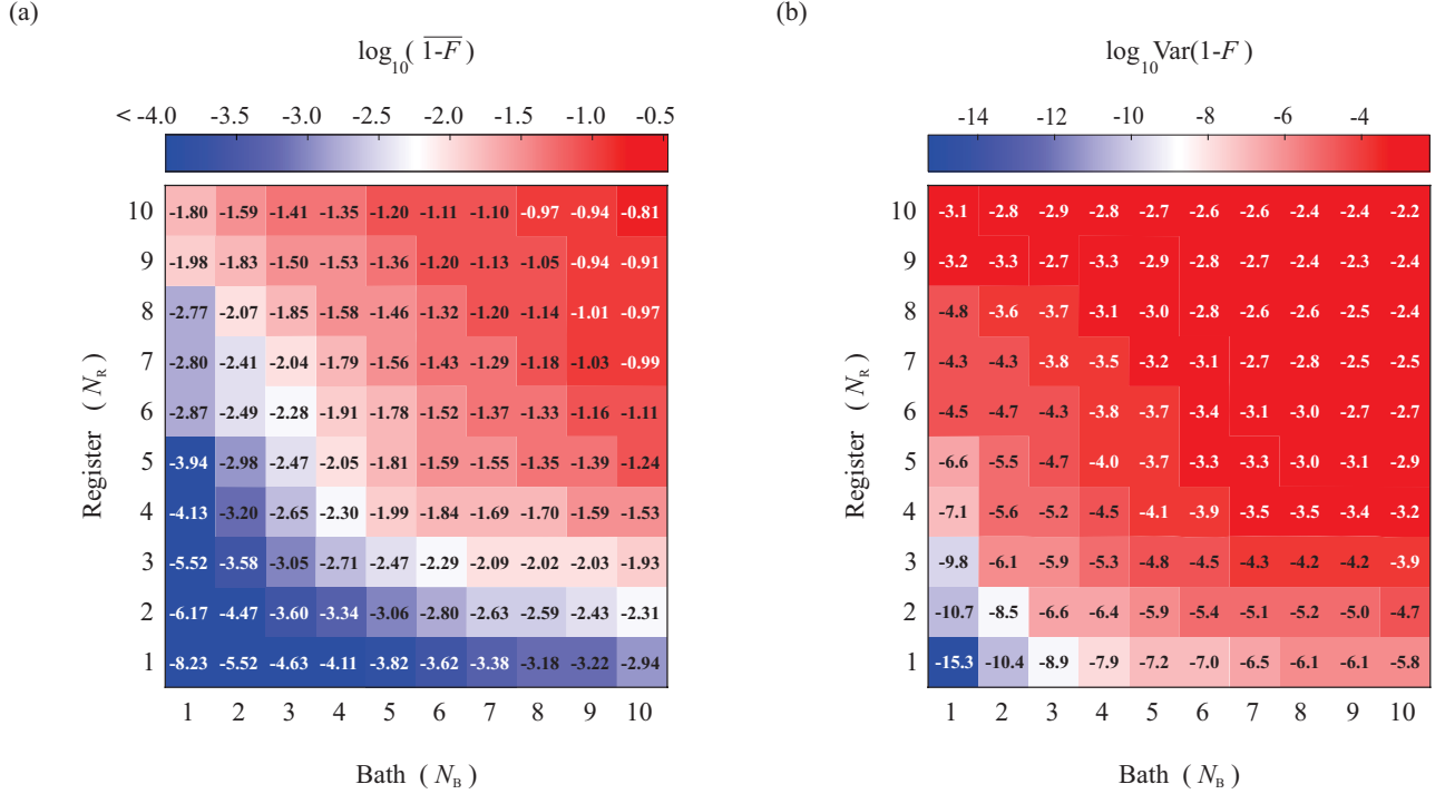
FIG. 6. Gate infidelity ( 1 - F ) versus the size of the bath (unwanted spins) and the size of the register (wanted or target spins) upon optimization over single-qubit rotations on the electronic spin. In (a) we plot the decimal logarithm of the statistical average of infidelity, i.e., \log_{10}(\overline{1-F}) , while in (b) we plot the variance of the infidelity on the same logarithmic scale \log_{10} \text{Var}(1-F) . The numbers in each tile give the value of \log_{10}(\overline{1-F}) and \log_{10} \text{Var}(1-F) , respectively. In the above simulations, we considered SiC samples with a silicon divacancy with total spin S = 1 , and the electron qubit is defined by (s_0, s_1) = (0, -1) . The HF values for the ^{13}\text{C} and ^{29}\text{Si} nuclei were drawn from uniform distributions in the intervals 2\pi[10, 200] kHz and 2\pi[0.5, 200] kHz, respectively. The entangling power threshold was set to \epsilon_p^{\text{th}} = 0.85 , the magnetic field is B = 584\text{G} leading to Larmor frequencies (\omega_L^C, \omega_L^{Si}) = 2\pi(625.37, -494.35) kHz, and the relative abundance was kept constant for all the cases, i.e., \frac{^{29}\text{Si}}{^{13}\text{C}} = \frac{4.7\%}{1.1\%} = 4.27 . Every data point on the heatmaps was obtained from 100 realizations, and for each trajectory we kept the combination (\tau, N) that resulted in the lowest maximum unwanted one-tangle.
