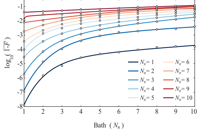
FIG. 5. Statistical average of the infidelity (circles) and fits (solid lines) versus the spin bath size. The lines are fits of the function \log_{10}(1 - F_{N_R}) = a_{N_R} e^{b_{N_R} N_B} + c_{N_R} e^{d_{N_R} N_B} to the collected data (circles). Each line refers to a different register size N_R , and the respective fitting parameters a, b, c, d are given in Table I.
