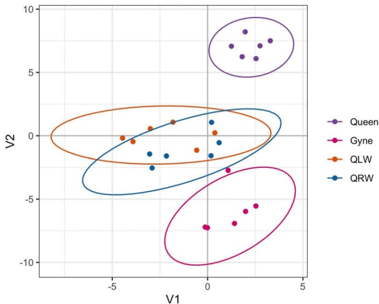
Fig. 2. – t-SNE plot showing clustering of Dufour's gland RNAseq samples based on treatment group using all gene expression data.
