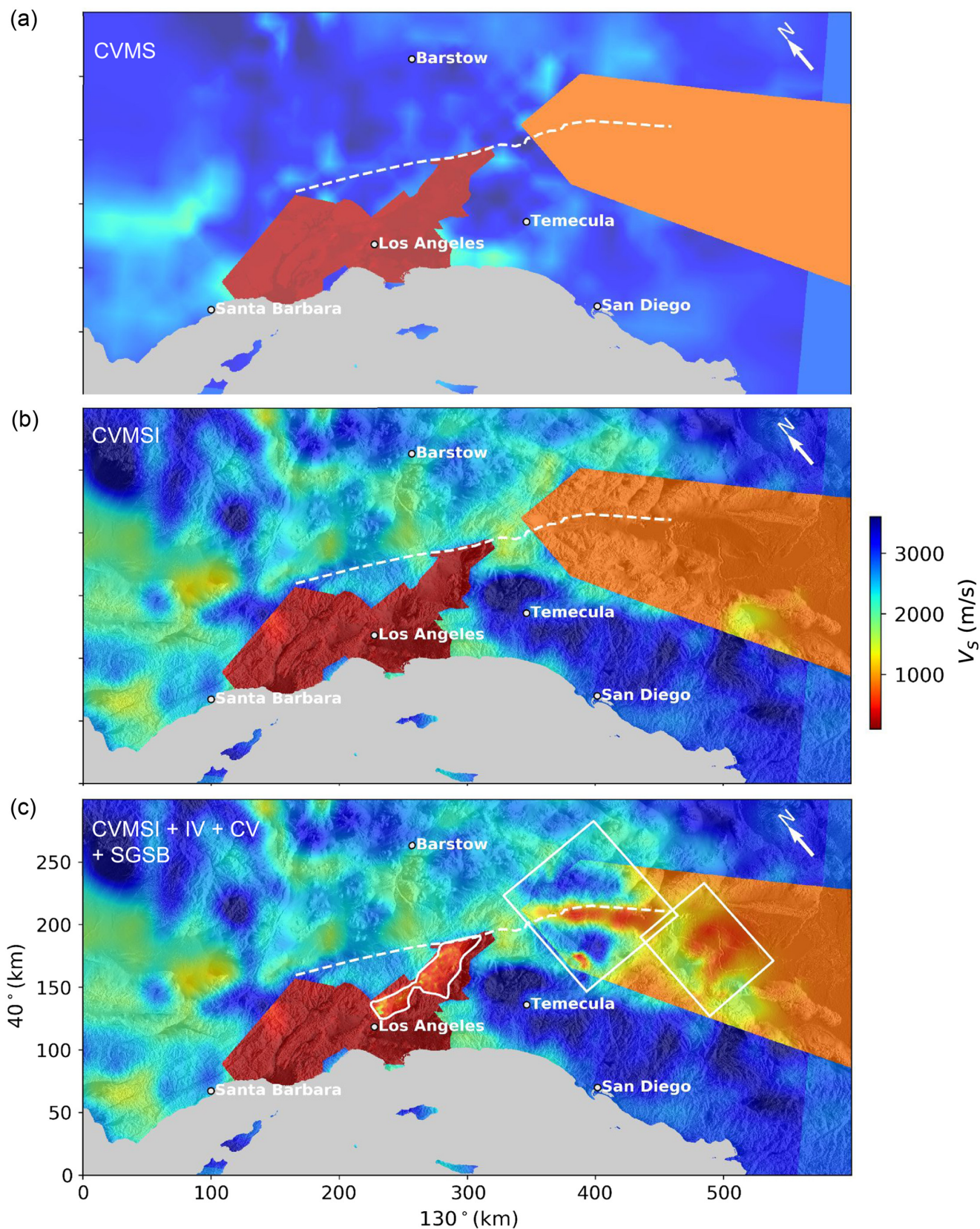
Figure 2. V_s at the free surface within the simulation domain for (a) Community Velocity Model version S4 (CVMS), (b) CVM-S4.26.M01 (CVMSI), and (c) CVMSI with local high-resolution models incorporated, with the fault trace depicted by a dashed
