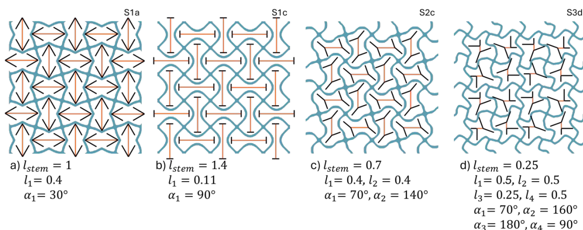
Figure 2. Exemplary 2D lattice geometries and their architectural parameters.
