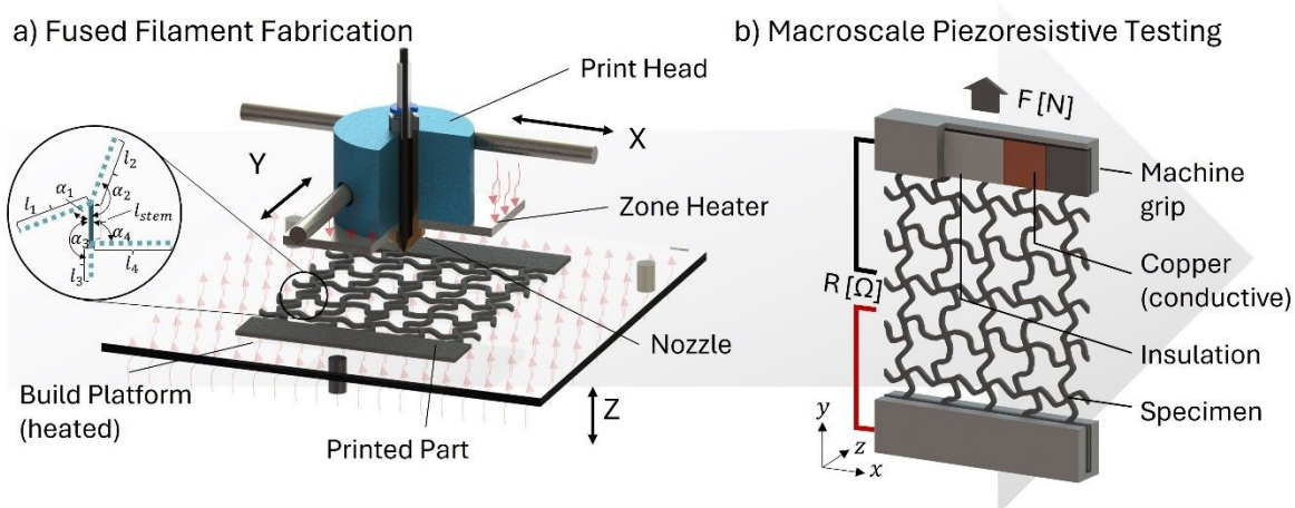
Figure 3. Schematic of a) FFF additive manufacturing process and b) Macroscale piezoresistive testing. On the left, an FFF setup with a heated platform and a moving print head dispensing material in predefined patterns is shown. The inset illustrates the parametrised BSB structure employed for generating the lattice design. On the right, is the configuration for tensile testing of printed lattice structures, including resistance measurements under strain. This setup ensures electrical isolation of the specimen with a non-conductive layer and optimal electrode contact via a copper layer.
