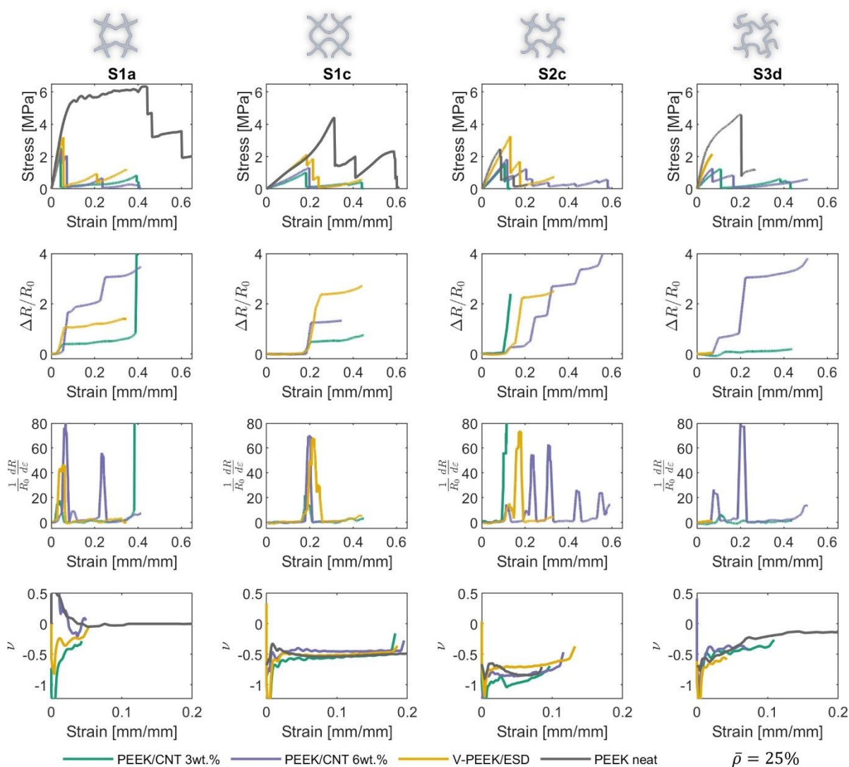
Figure 6. 2D auxetic PEEK/CNT lattice structures of the same relative density (25%) under tensile loading. Row 1: stress-strain response, row 2: relative change in resistance as a function of strain, row 3: (1/R_0)(dR/d\epsilon) as a function of strain, and row 4: Poisson's ratio as a function of strain until first ligament failure.
