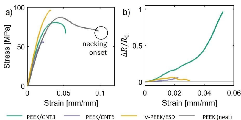
Figure 5. Representative graphs of parent PEEK and PEEK nanocomposites under tensile loading: a) engineering stress-strain response, where strain is measured by DIC, showing the region where necking occurs for neat PEEK and b) fractional change in resistance as a function of strain for three PEEK nanocomposites.
