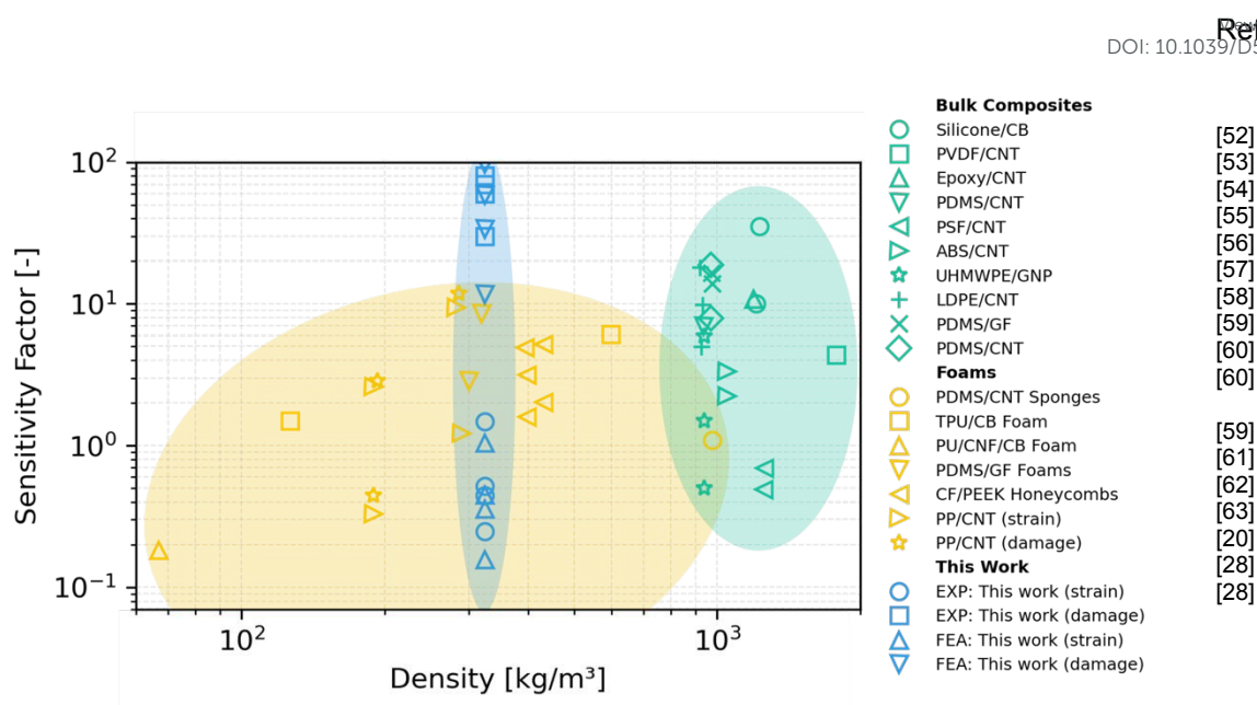
Figure 10. Assessment of sensitivity factors in AM-enabled V-PEEK/ESD 2D auxetic lattice nanocomposites versus extant piezoresistive materials [20,28,52–63].
