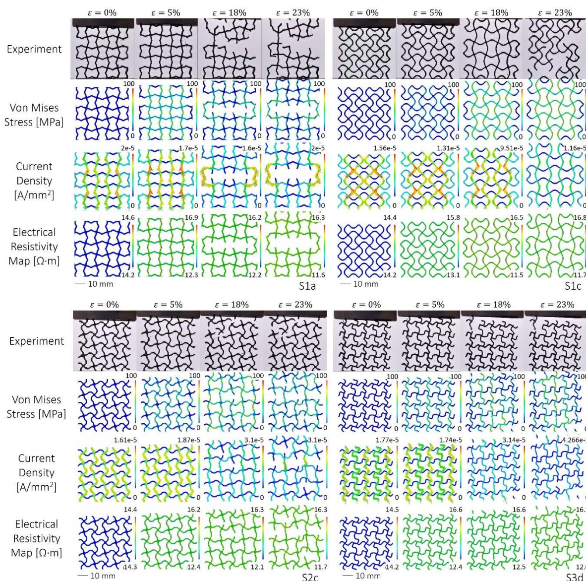
Figure 8. Comparative assessment of deformation and failure behaviour of nanoengineered auxetic structures under tensile loading: This figure presents a series of experimental and simulated visualisations for various auxetic PEEK/CNT lattice structures (S1a, S1c, S2c, S3d) at different strain levels (0%, 5%, 18%, 23%). The first row for each specimen type displays the experimental images of the deformed structures. The subsequent rows showcase the corresponding simulated maps with Von Mises stress distribution, current density, and electrical resistivity, respectively. The colour-coded scales indicate the magnitude of the respective physical quantities, providing an insight into the mechanical and electrical responses of the auxetic lattices during deformation.
