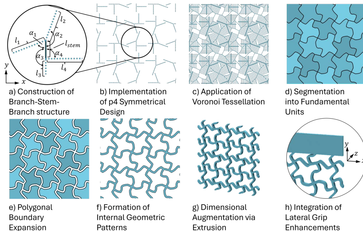
Figure 1. Sequential design and transformation process for the generation of 2D auxetic structures with a relative density \bar{\rho} = 25\% : a) construction of a branch-stem-branch (BSB) structure, b) implementation of p4 symmetry, c) application of Voronoi tessellation, d) segmentation into fundamental units, e) polygonal boundary expansion, f) formation of internal geometric patterns, g) dimensional augmentation via extrusion, and h) integration of lateral grip enhancements.
