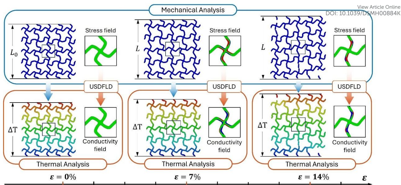
Figure 4. The flowchart depicts the methodology of piezoresistive finite element analysis. The electrical resistivity results were derived using the electrical-thermal analogy within steady-state thermal analyses synchronized with mechanical analysis time steps. The modification of local electrical conductivity was based on the stress field obtained from mechanical analysis in the thermal analysis, utilizing the USDFLD subroutine to capture the piezoresistive effect of the composite material.
