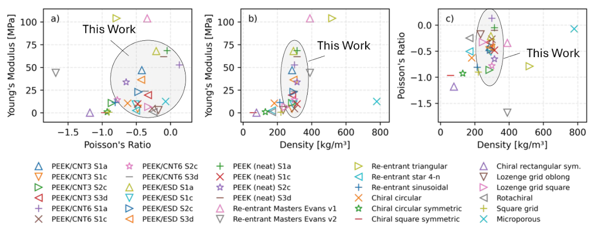
Figure 9. Chart of experimentally evaluated material properties of the 2D auxetic structures analysed in this study compared to FE predictions reported on extant auxetic structures, showing density, Young's modulus and Poisson's ratio (all external sources are summarised here): Comparative study of auxetic geometries using computer-aided design and engineering by J. Elipe and A. Lantada [51]
