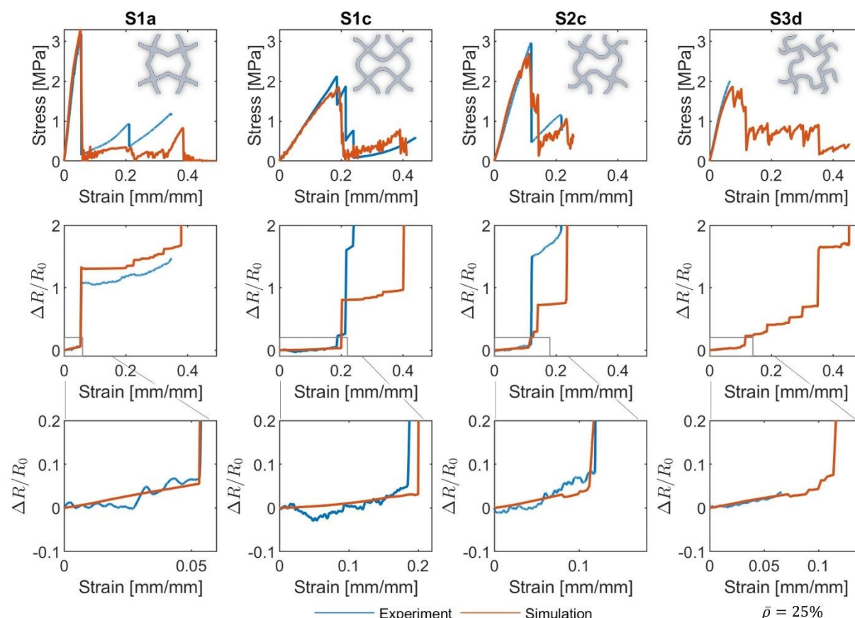
Figure 7. Mechanical and piezoresistive performance comparison of experimental (representative) and simulation results for auxetic PEEK/CNT lattices of the same relative density (25%) under tension: The figure illustrates four sets of graphs (S1a, S1c, S2c, S3d) depicting the stress-strain response and relative resistance change ( \Delta R/R_0 ) as a function of applied strain. The top row presents stress-strain curves, the middle row shows the overall \Delta R/R_0 response, and the bottom row provides a detailed view of \Delta R/R_0 at lower strains. Experimental data (orange) and model predictions (blue) are juxtaposed to demonstrate the predictive capability of the proposed piezoresistive model.
