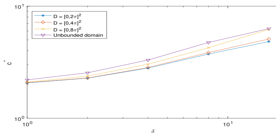
Figure 14. Log-log plot of c^* vs. \delta as domain size increases, \epsilon = 0.5 , 2D random cellular flow.
