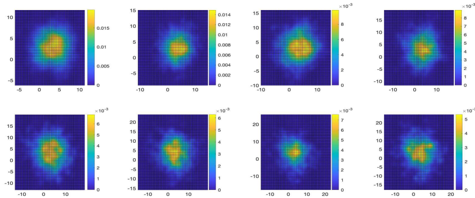
Figure 15. Particles distribution under dynamic shift, t = 8 to t = 64 , e = (1, 0) .
