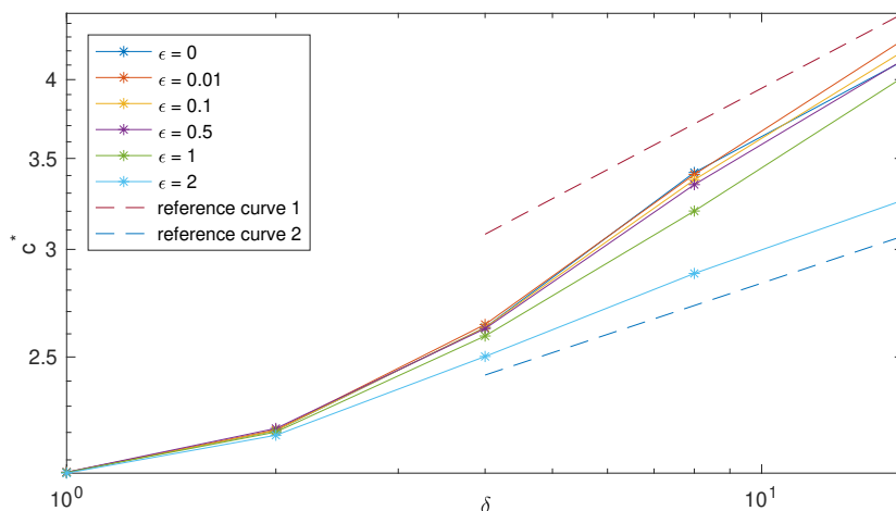
Figure 7. Log-log plot of c^* vs. \delta in 2D random cellular flow at different \epsilon ; z = (1, 0) .
