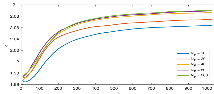
Figure 2. Front speed c^* vs. t of random shear flow with different Fourier modes N_F .
