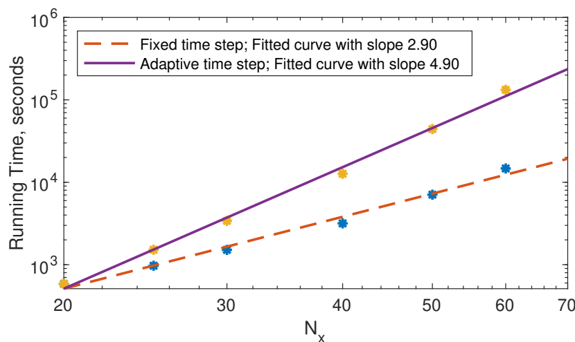
Figure 6. Log-log plot of mesh size N_x vs. running time.
