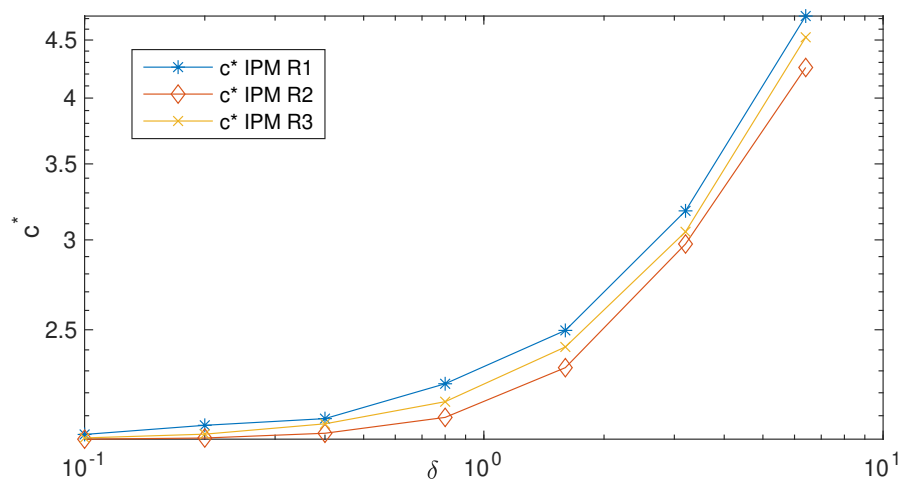
Figure 10. Log-log plot of c^* vs. \delta , z = (0, 1) , 2D random shear flow by IPM.
