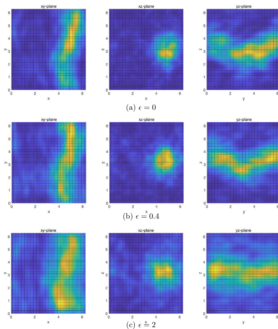
Figure 18. Three planar views of particle distributions for randomly perturbed ABC flow at \epsilon = 0, 0.4, 2 , showing increased blurring/broadening effect of perturbations.
