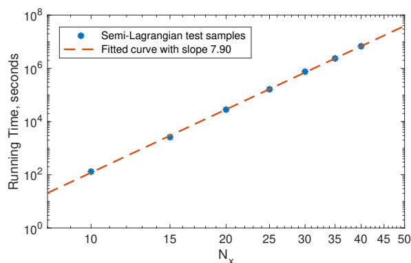
Figure 5. Log-log plot and table of mesh size N_x vs. running time of SL + CN method in 3D cellular flow (* in the table means the time is estimated).
