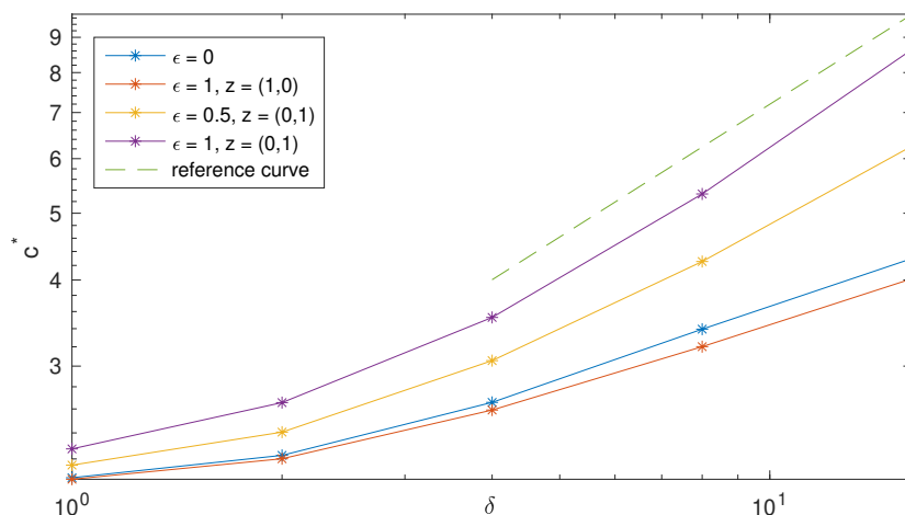
Figure 8. Log-log plot of c^* vs. \delta in 2D random cellular flow with different \epsilon and z .
