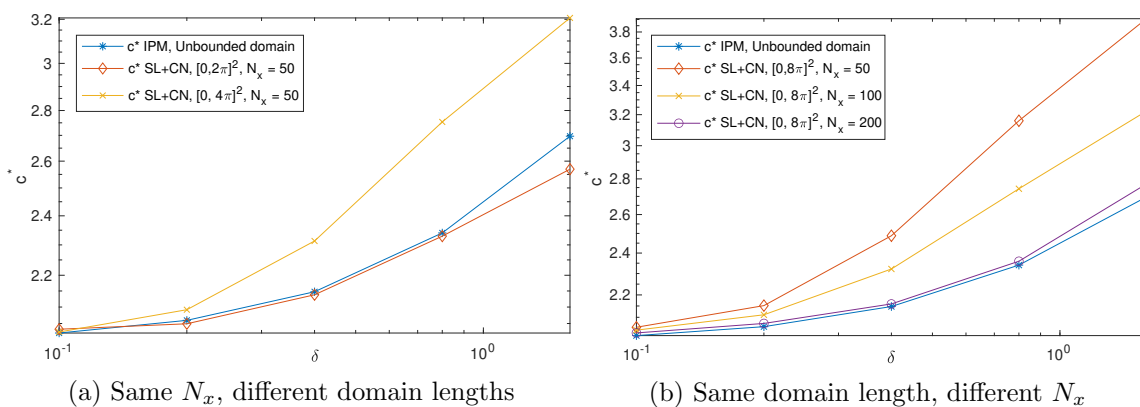
Figure 4. Comparison of c^* by IPM and SL + CN method.
