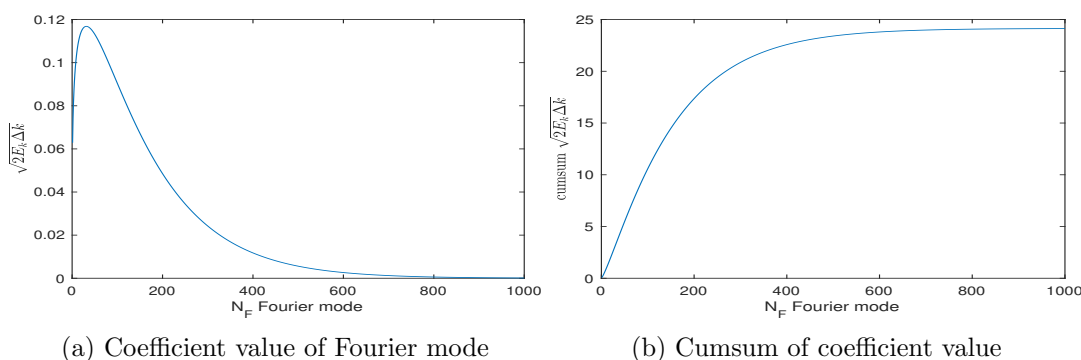
Figure 1. Performance of the coefficient of the generated random velocity field.
