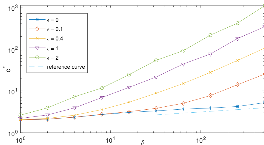
Figure 13. Log-log plot of c^* vs. \delta at different \epsilon , 3D random cellular flow.
