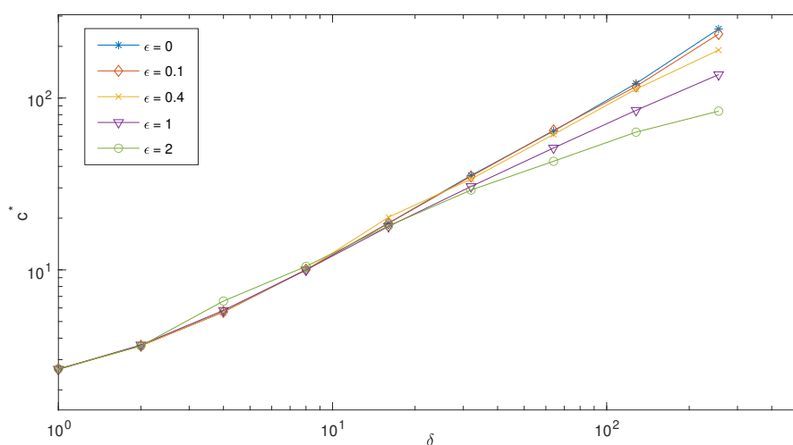
Figure 12. Log-log plot of c^* vs. \delta with different \epsilon , 3D random ABC flow.
