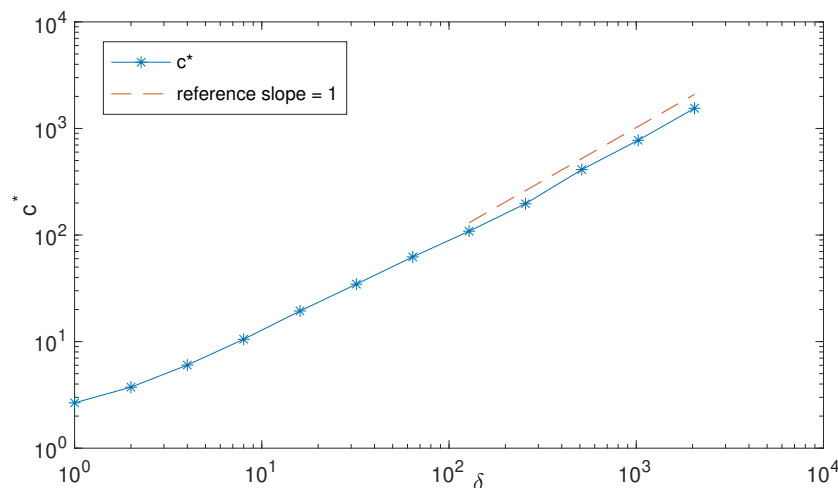
Figure 11. Log-log plot of c^* vs. \delta , \epsilon = 0 , z = (0, 1, 0) , 3D ABC flow.
