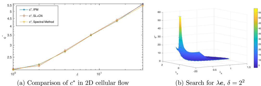
Figure 3. Computation of c^* in 2D cellular flow.
