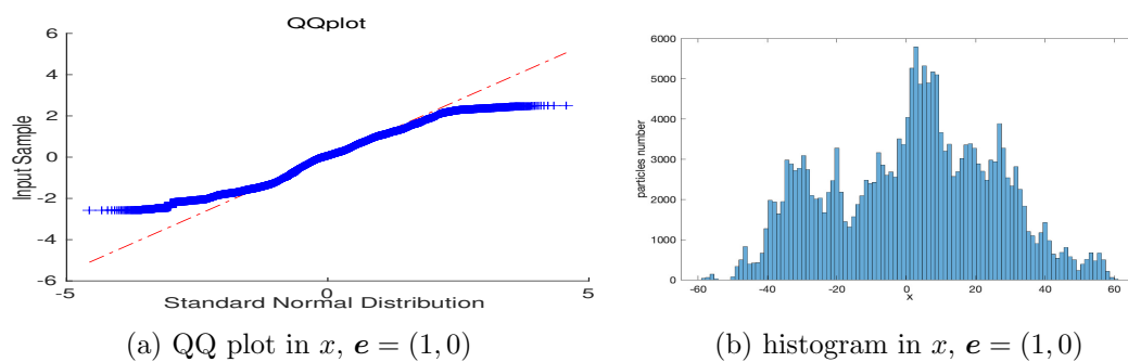
Figure 17. QQ plot and histogram plot for random shear flow, e = (1, 0) , t = 1024 .
