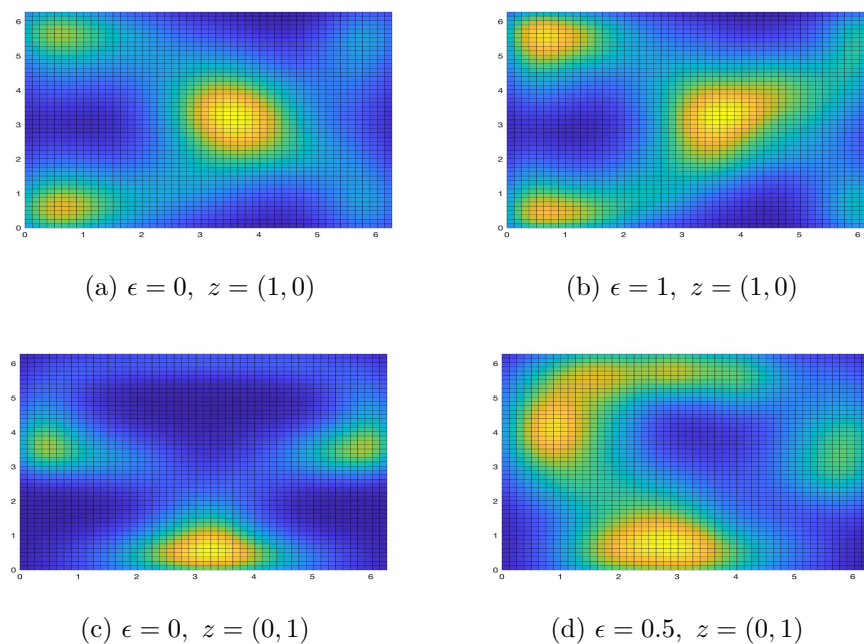
Figure 9. Comparison of invariant measure in 2D (random) cellular flow.
