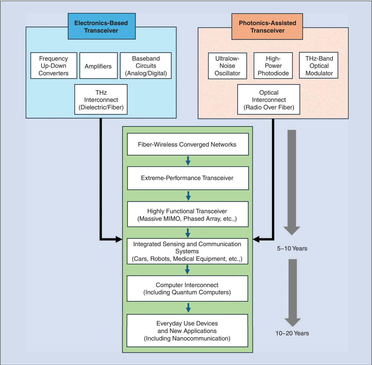
FIGURE 3 Key devices that constitute electronics- and photonics-based transceivers, and the evolution of application technologies resulting from their integration and convergence. MIMO: multiple-input multiple-output.
