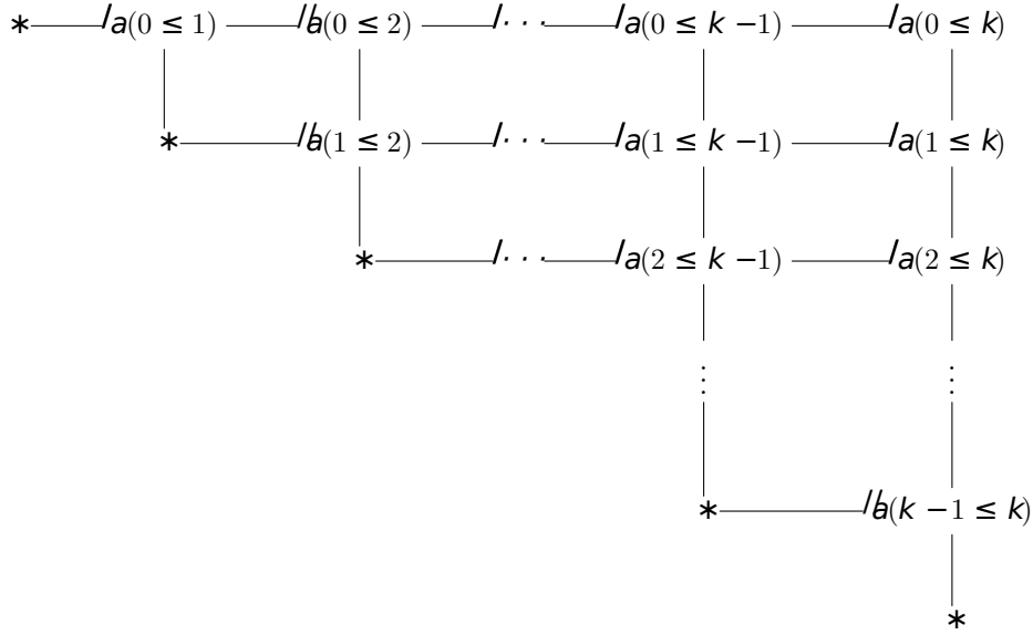
Fig. 5.9: A k -simplex in S_k C_0
