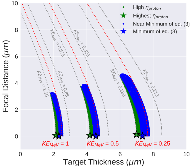
FIGURE 6 | Parameters that produce maximum proton energy cut-offs in three different desired ranges: 1.0, 0.5, and 0.25 MeV. Combinations of thickness and focal distance that produce these energy cutoffs (irrespective of the laser-to-proton conversion efficiency) are shown with dotted red lines. With each red line we also show with dotted gray lines the thicknesses and focal distances that produce proton energy cutoffs that are +15% or −15% of the cutoff goal. Green shaded areas show regions where the laser-to-proton conversion efficiency is high (i.e., within 5% of the optimal value). A green star shows the ideal conditions for maximizing the proton conversion efficiency. The blue region corresponds to using all the terms in Equation (3) and the blue star indicates the ideal conditions according to that minimization scheme.
