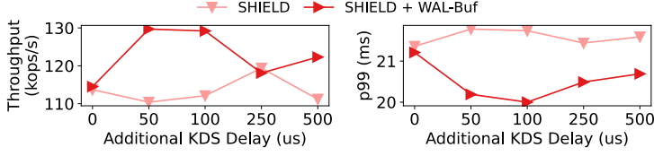
Fig. 16. Impact of KDS Latency.
