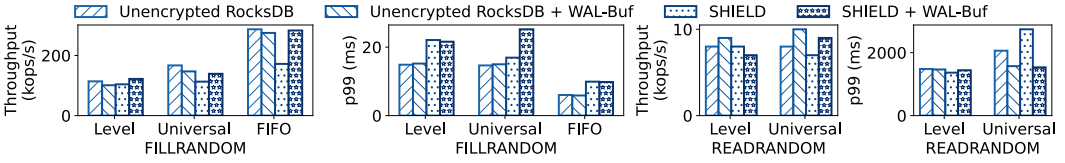
Fig. 15. Different Compaction Policies.
