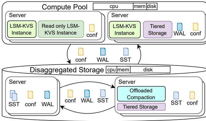
Fig. 2. Different LSM-KVS Deployments in DS.
