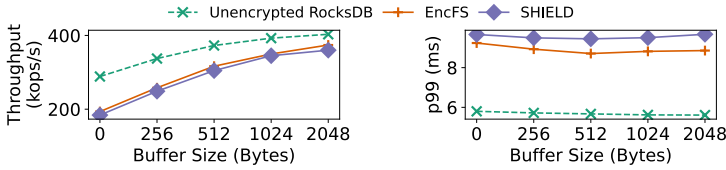
Fig. 14. Sensitivity to Buffer Sizes.
