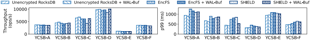
Fig. 9. Throughput and P99 Latency for YCSB Tests in a Monolith Server.
