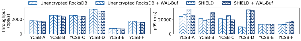
Fig. 21. YCSB Results with Disaggregated Storage
