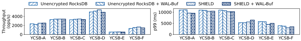
Fig. 24. YCSB Results with Offloaded Compaction.
