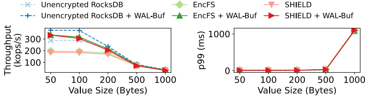
Fig. 10. Sensitivity to Value Sizes.
