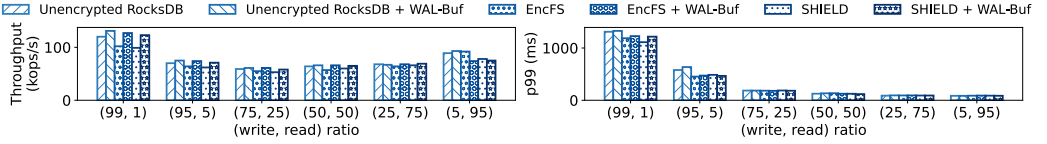
Fig. 8. Throughput and P99 Latency for Different Read and Write Ratios in a Monolith Server.
