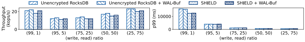
Fig. 20. Throughput and P99 Latency for Different Read and Write Ratios in Disaggregated Storage.
