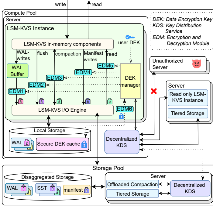
Fig. 6. Design Overview for SHIELD.
