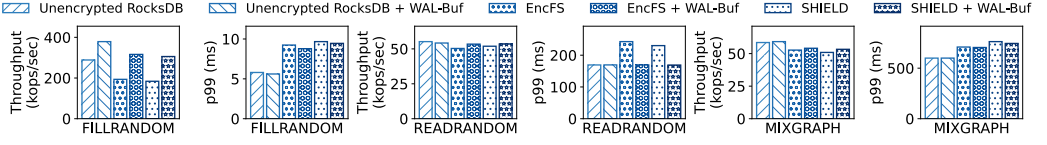
Fig. 7. Baseline Results in a Monolith Server.
