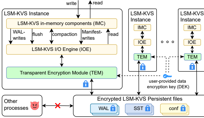
Fig. 5. Design Overview for Instance-level Encryption.
