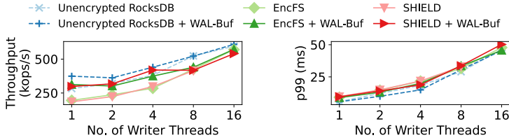
Fig. 11. Sensitivity to Writer Threads.
