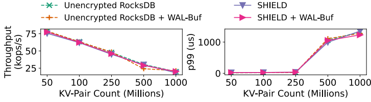
Fig. 17. Increasing Dataset sizes.
