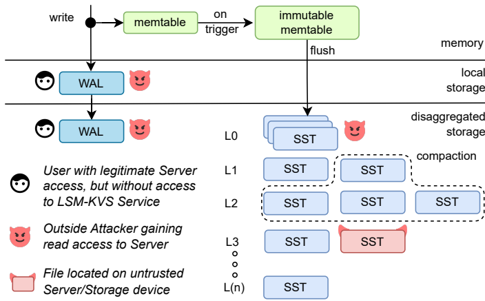
Fig. 3. Security Threats Considered in the Threat Model.
