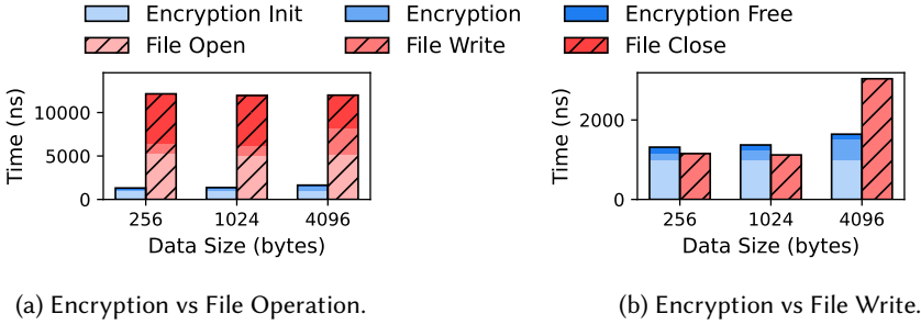
Fig. 4. Analysis of Encryption Costs and Writes. 2
