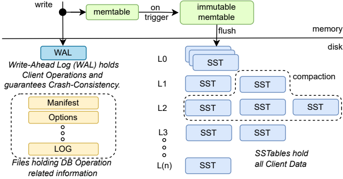
Fig. 1. Different Components involved in Writes for KV-Pairs in LSM-KVS.
