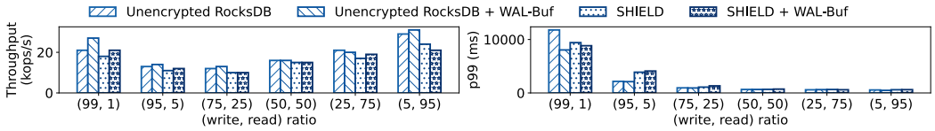
Fig. 23. Throughput and P99 Latency for Different Read and Write Ratios with Offloaded Compaction.
