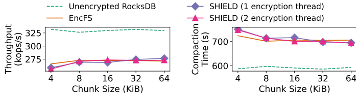
Fig. 13. Sensitivity to Chunk Sizes and Encryption Threads.
