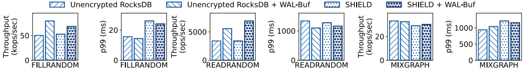
Fig. 19. Baseline Results with Disaggregated Storage.
