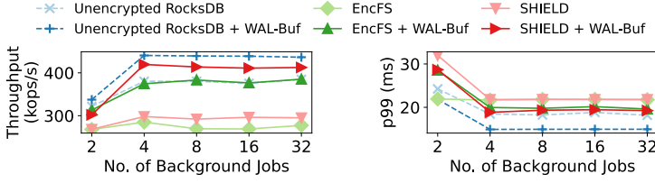
Fig. 12. Sensitivity to Background Threads.
