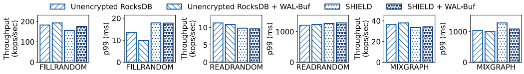
Fig. 22. Baseline Results with Offloaded Compaction.
