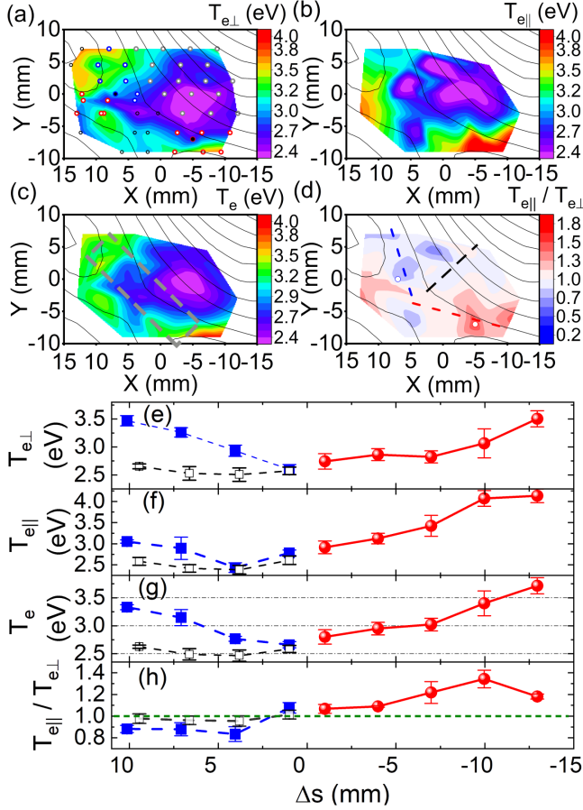
FIG. 3. 2D spatial profile of (a) perpendicular electron temperature T_{\perp} , (b) parallel electron temperature T_{\parallel} , (c) effective electron temperature T_e and (d) anisotropy T_{\parallel}/T_{\perp} . Black lines are in-plane magnetic field projections, and 43 dots show the measurement locations, grouped into regions around the separatrix I (red), II (blue), and the inflow (gray). The dashed rectangle in (c), half of the electron diffusion region, is used to calculate energy fluxes. The corresponding 1D profiles along separatrix I [red points for the red dashed line in (d)], II [blue solid squares for the blue dashed line in (d)] and the inflow direction [black open squares for the black dashed line in (d)]: (e) T_{\perp} , (f) T_{\parallel} , (g) T_e , and (h) T_{\parallel}/T_{\perp} . \Delta s is the distance from the X point at (x, y) = (5 \text{ mm}, -3 \text{ mm}) .
