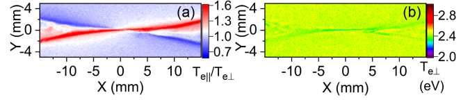
FIG. 4. (a) T_{\parallel}/T_{\perp} and (b) T_{\perp} in the reconnection plane obtained from a 2D PIC simulation.
