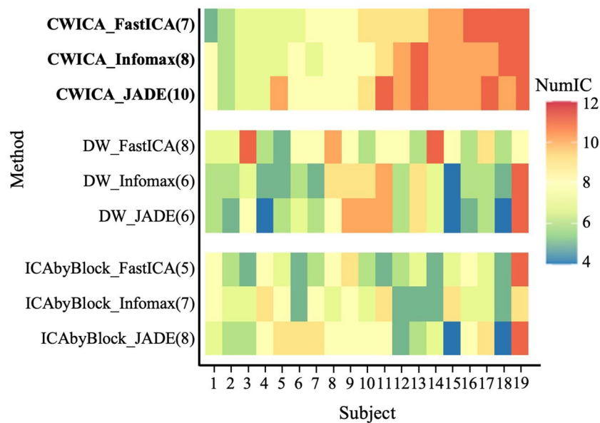
Figure 7. Heatmap of estimated number of ICs. Each column describes the estimated number of ICs by 9 methods from the same subject. Most estimated number of ICs are around 7 to 12, which indicates the number of sources contained in raw EEG signals. The value in parentheses represents the most frequency result of each method.
