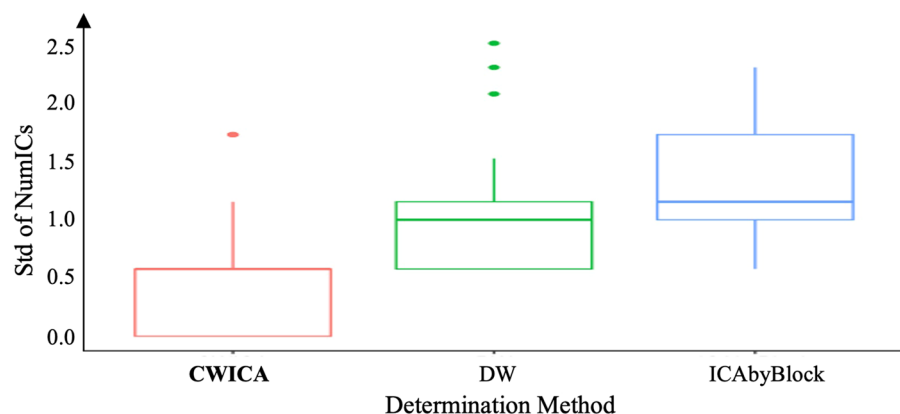
Figure 8. Precision comparison of the estimated number of ICs for three determination methods for every individual.
