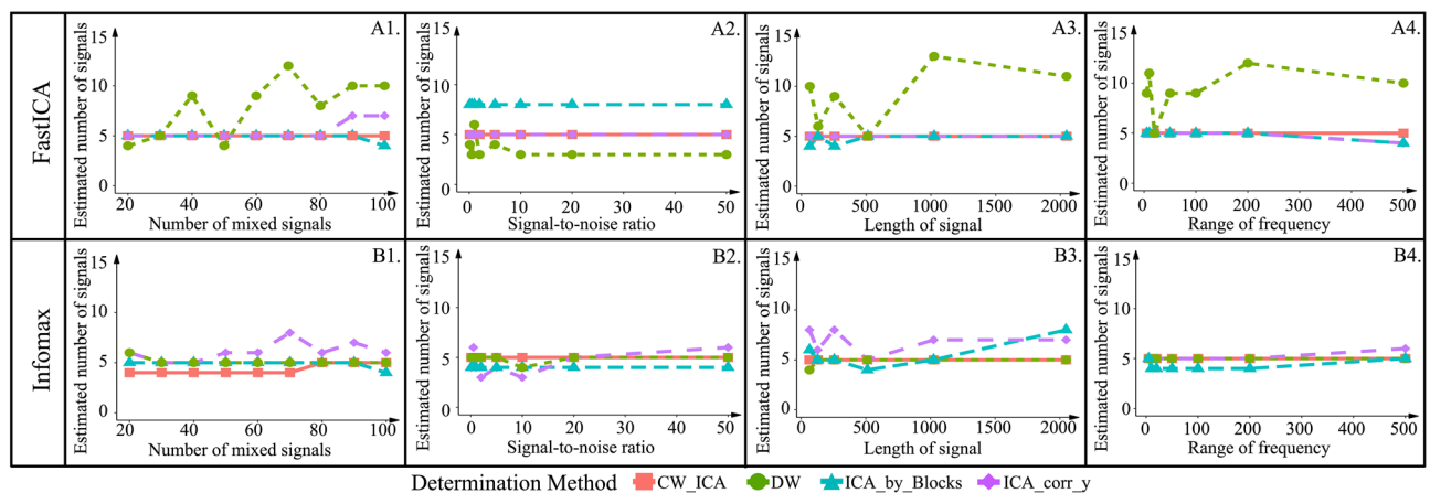
Figure 6. Estimated number of source signals with variety parameters in mixed signals.
