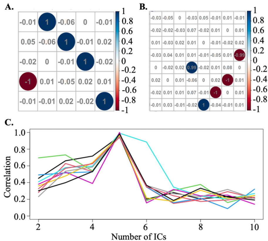
Figure 2. (A) Off-diagonal correlation plot for estimated ICs from two blocks ( q=5 ). (B) Off-diagonal correlation plot for estimated ICs from two blocks ( q=8 ). (C) Signal-correlation plot of one replicate. The significant drop at 5th indicates the optimal number of ICs is 5 at this replicate.
