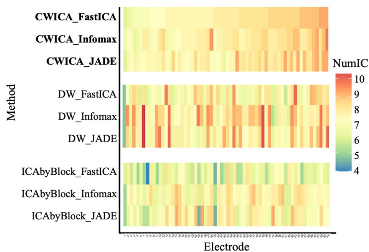
Figure 10. Heatmap of estimated number of ICs. Each column describes the estimated number of ICs by 9 methods at the same electrode.
