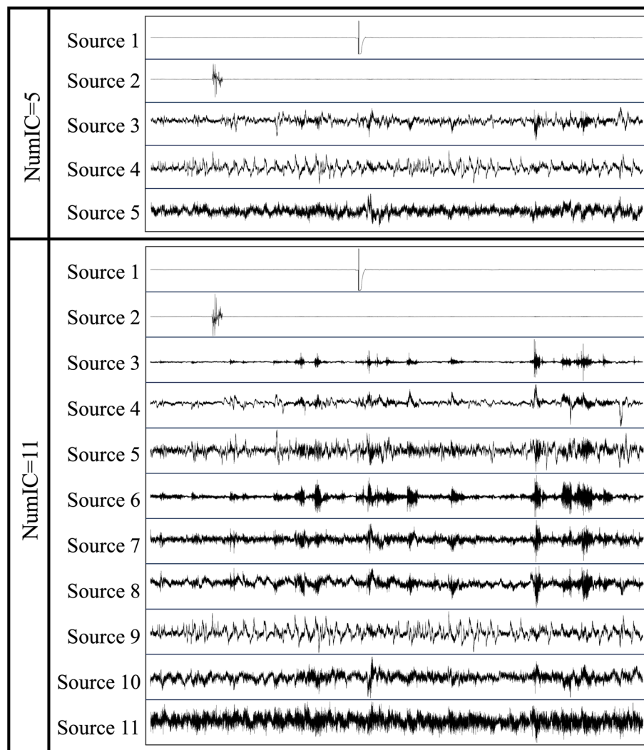
Figure 9. Extracted EEG source signals from subject 18 with different number of ICs.
