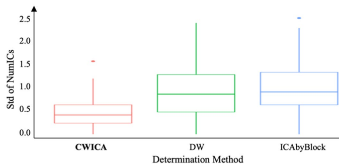
Figure 11. Precision comparison of the estimated number of ICs for three methods of determining the number of ICs for each channel over all 19 individuals.
