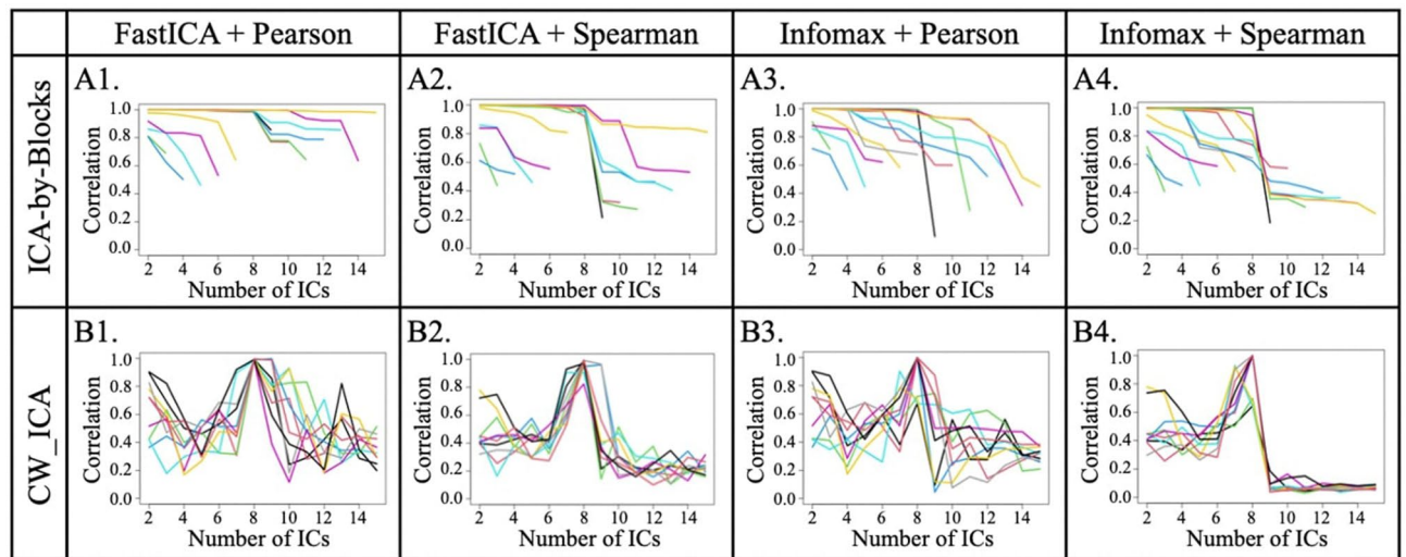
Figure 4. Signal-Correlation plots for (A) ICA-by-Blocks and (B) CW_ICA methods.
