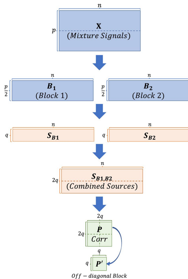
Figure 1. Stages of data structures in CW_ICA method.
