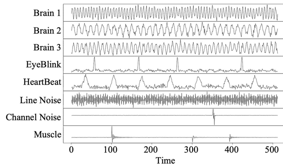
Figure 3. Plots of simulated EEG component signals. The signal length is set as 512.
