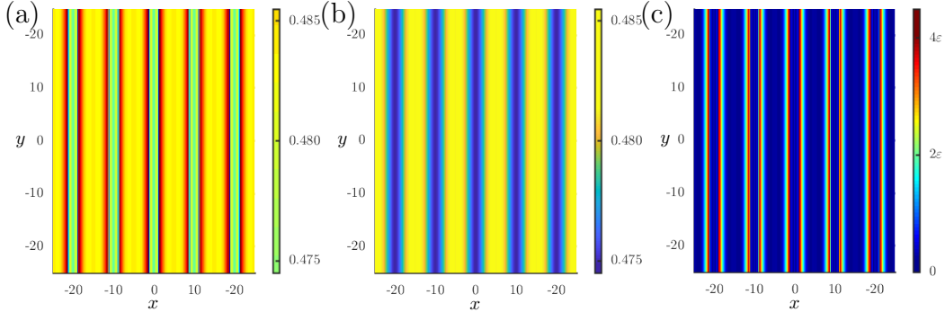
Figure 4: (a) The surface \mu_{\text{esc}}(x, y) , shown here in the projection onto the (x, y) plane, is where the hard onset of oscillations occurs. It has been obtained from numerical simulation of (1) with stripe source term I_S(x, y) (34) and constant initial data A_0(x, y) = 1 given at \mu_0 = -1 . (b) The buffer surface \mu_{\text{buf}}(x, y) defined by (19), with g given by the linear combination of (20) and (27). (c) The difference |\mu_{\text{esc}}(x, y) - \mu_{\text{buf}}(x, y)| . The parameters are d = 1 , \omega_0 = 0.5 , \alpha = 0.2 , and \varepsilon = 0.01 .
