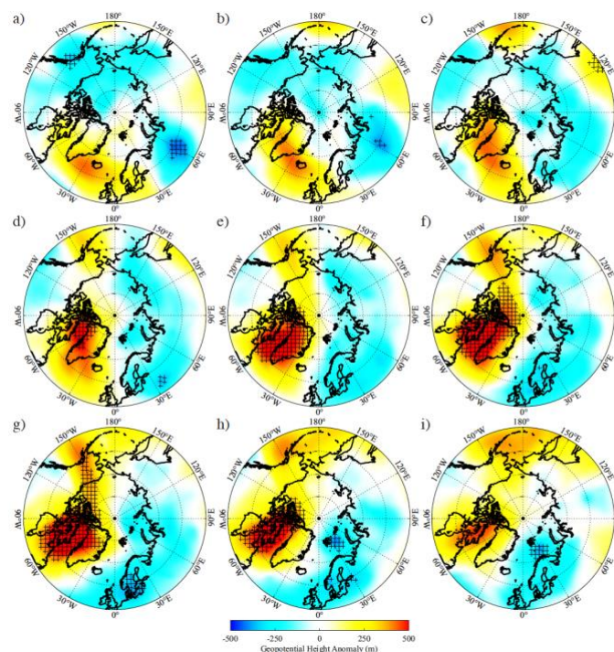
Figure 6. 500 hPa geopotential height ( z500 ) anomaly (m) from the ERA5 at 0 GMT on: a) 2 March, b) 3 March, c) 4 March, d) 5 March, e) 6 March, f) 7 March, g) 8 March, h) 9 March, and i) 10 March 2023. The anomalies are presented with respect
