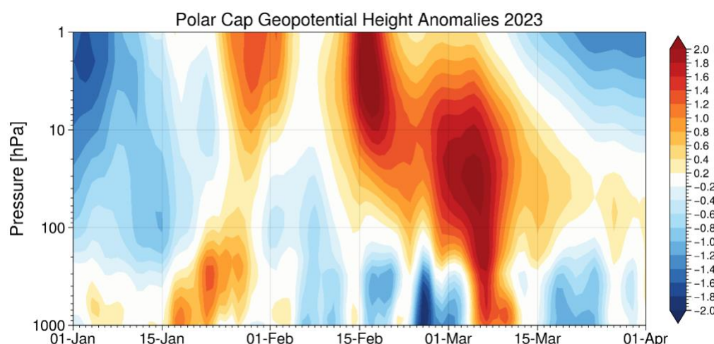
Figure 4. Polar cap (60-90°N) standardized geopotential height anomalies (unitless) from the surface to the upper stratosphere during winter 2023. The standardized anomalies are calculated at each pressure level by removing the daily climatology and dividing by the daily standard deviation. The standardized anomalies are shown relative to the day of year for the 1979-2023 period of the ERA5 reanalysis.
